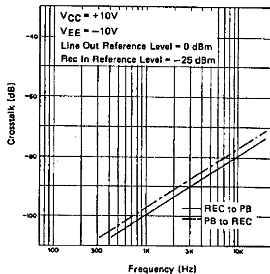
Recording and play back crosstalk
