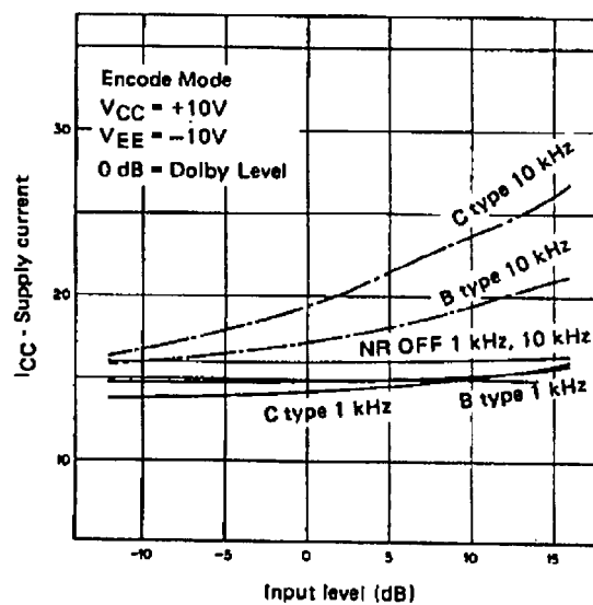
Supply current vs. Input level
