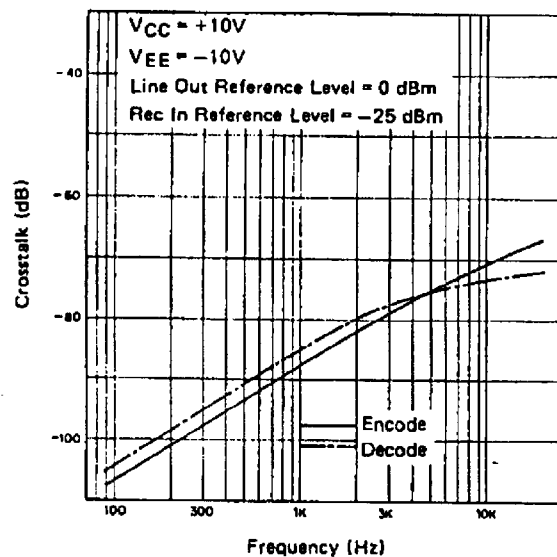
Channel to channel crosstalk
