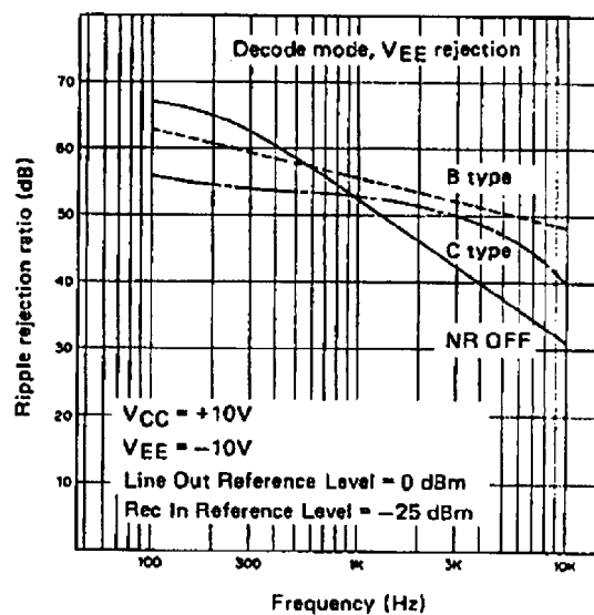
Ripple rejection ratio (4)
