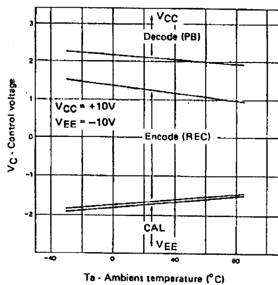
Control threshold voltage (2)
