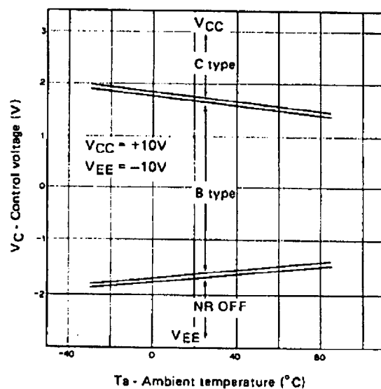
Control threshold voltage (1)
