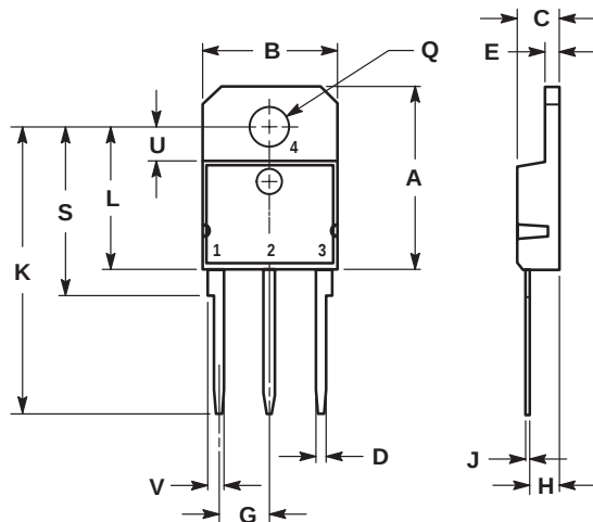
CASE 340D-01 (TO-218)
