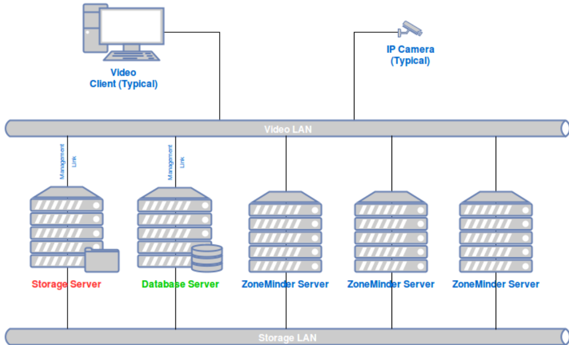
ZoneMinder Multi-Server Network Topology
