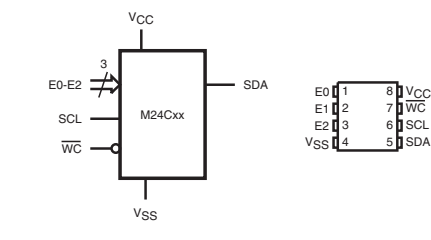
IC102: M24C02-RDW6TP 2 K-bit and 1 K-bit serial I2C bus EEPROM
