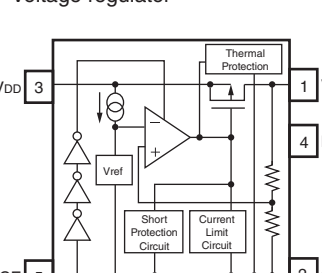
IC109: R1154H058B-T1-F Voltage regulator
