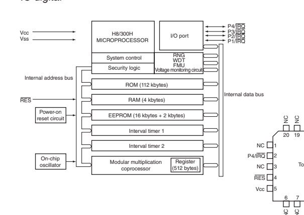
IC103: MF1341S1264 IC digital
