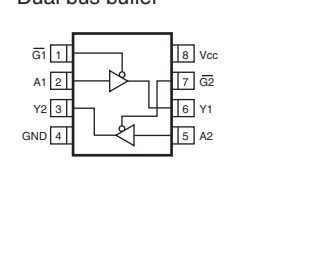
IC108: TC7WH125FK Dual bus buffer
