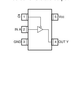
IC104, 107: TC7SZ125FU Bus buffer 3-state output
