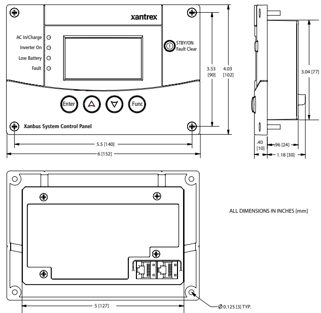
Figure 15 Xabus SCP Dimensions
