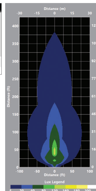
Eco Light Asymmetrical Lens Ground Pattern Birds Eye View
