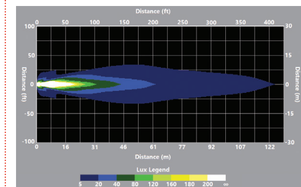
Eco Light Symmetrical Lens Cross Sectional Pattern
