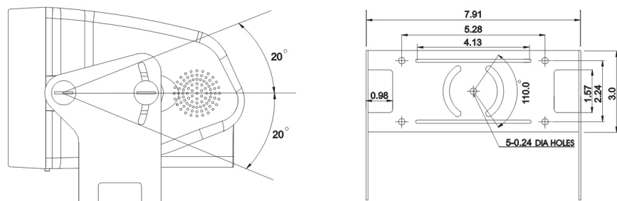
MONITOR MOUNTING HOLE PATTERN
