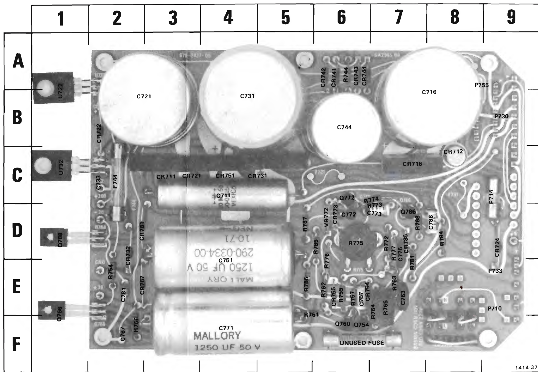
Fig. 7-17B. A3 Regulator circuit board below SN B050000.
