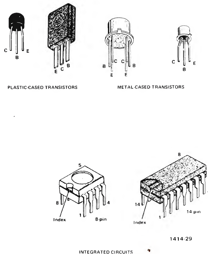
Fig. 7-10. Semiconductor lead configuration for Main circuit board.
