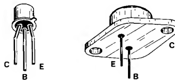
METAL-CASED TRANSISTORS
