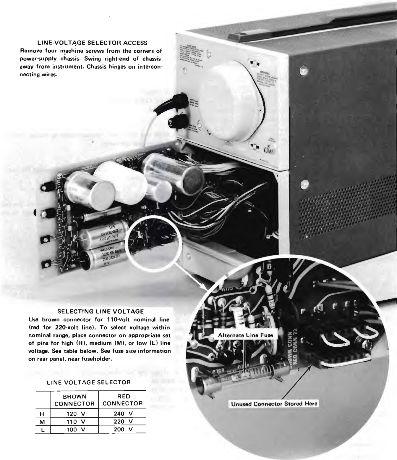
Fig. 4-1. Power transformer line-voltage taps.
