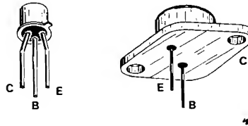
METAL-CASED TRANSISTORS
