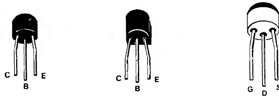
PLASTIC-CASED TRANSISTORS
