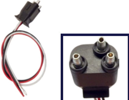
Straight - Tri-pole (T99-0010-1)
