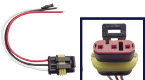
Straight - Amp Connection (T99-0040-1)
