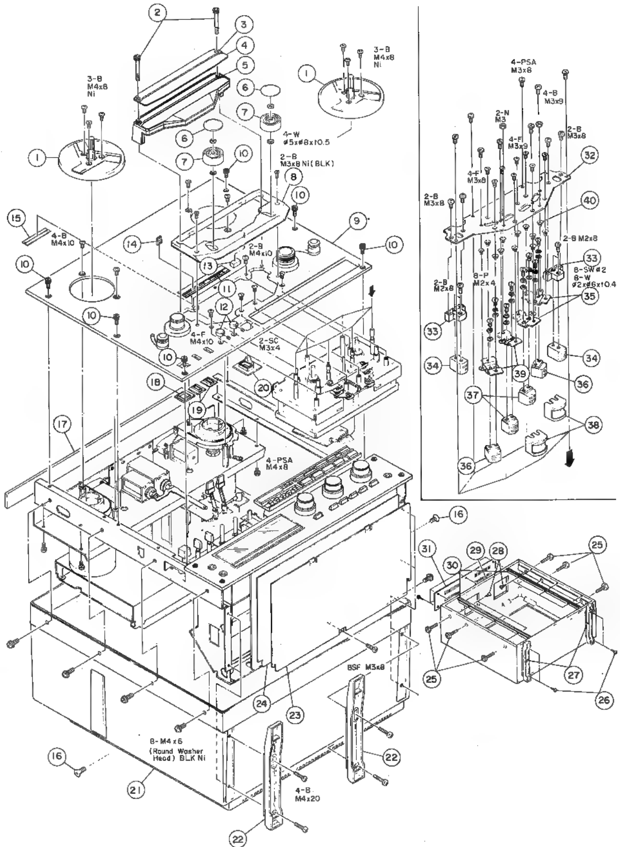
EXPLODED VIEW-1
