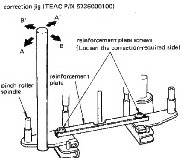
Fig. 2-18 Pinch roller/capstan alignment
