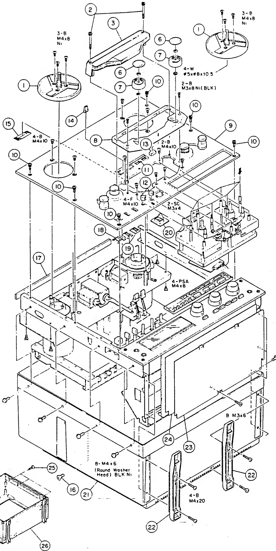
EXPLODED VIEW-1
