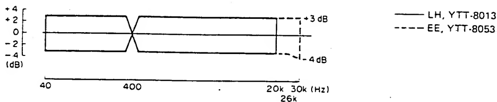
Fig. 3-7 Overall frequency response (19cm/s)
