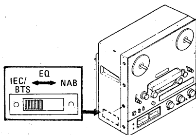
Fig. 3-6 EQ switch location (X-1000M only)
