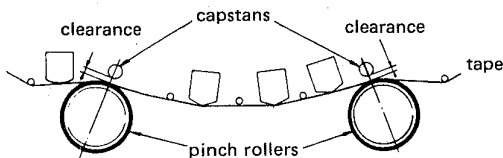
Fig. 2-4 Pause position adjustment
