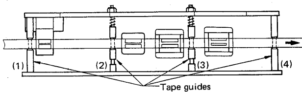
Fig. 2-14 Tape guide and head arrangement
