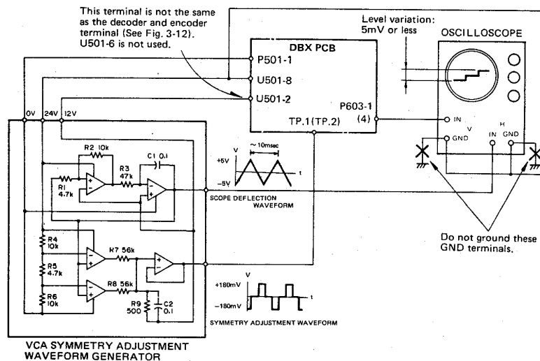
Fig. 3-14 VCA symmetry adjustment setup (decoder)
