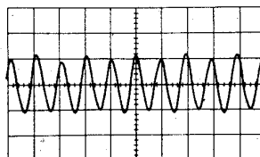
Fig. 3-10 RMS symmetry adjustment (correct)
