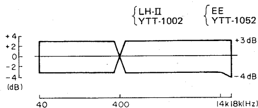
Fig. 3-4 Playback frequency response (9.5cm/s)
