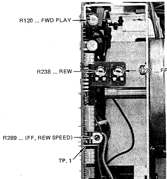
Fig. 2-9 Tape tension adjuster location
