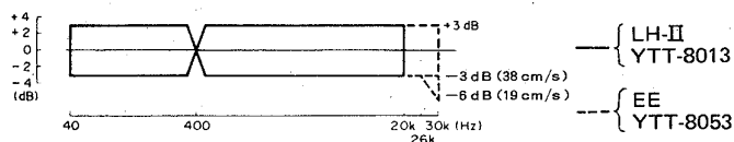
Fig. 3-8 Overall frequency response (38cm/s, 19cm/s)
