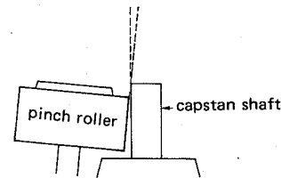
Fig. 2-16 View in direction A (example of non-parallelism)
