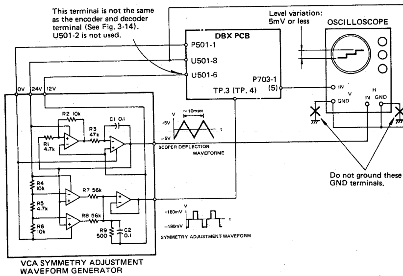
Fig. 3-12 VCA symmetry adjustment setup (encoder)
