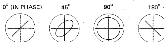
Fig. 3-3 Confirming phase relationship
