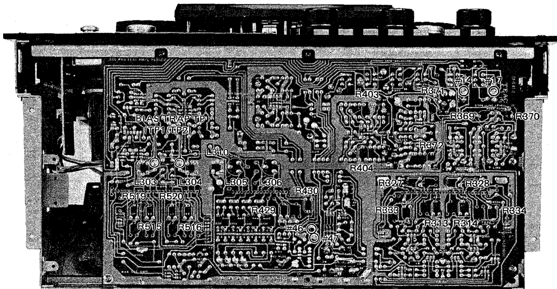
Fig. 3-15 REC AND PLAY AMP PCB
