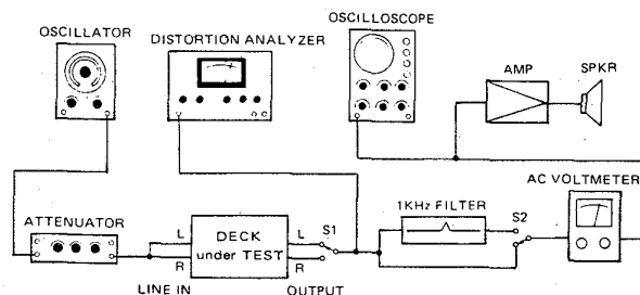
Fig. 3-1 Basic connection
