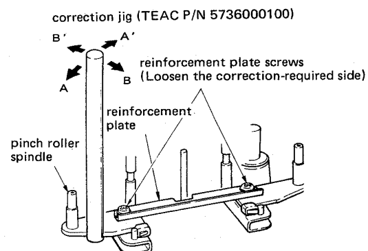
Fig. 2-18 Pinch roller/capstan alignment
