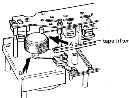
Fig. 2-15 Directions for pinch roller parallelism check
