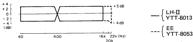
Fig. 3-7 Overall frequency response (9.5cm/s)
