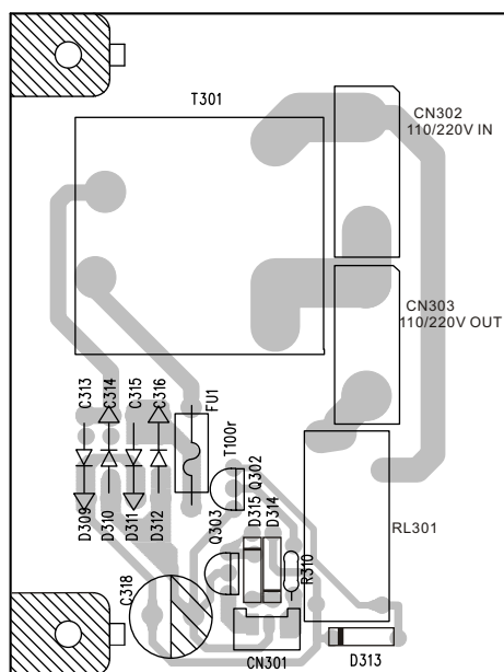
STANDBY PCB
