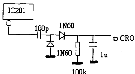
Detector circuit
