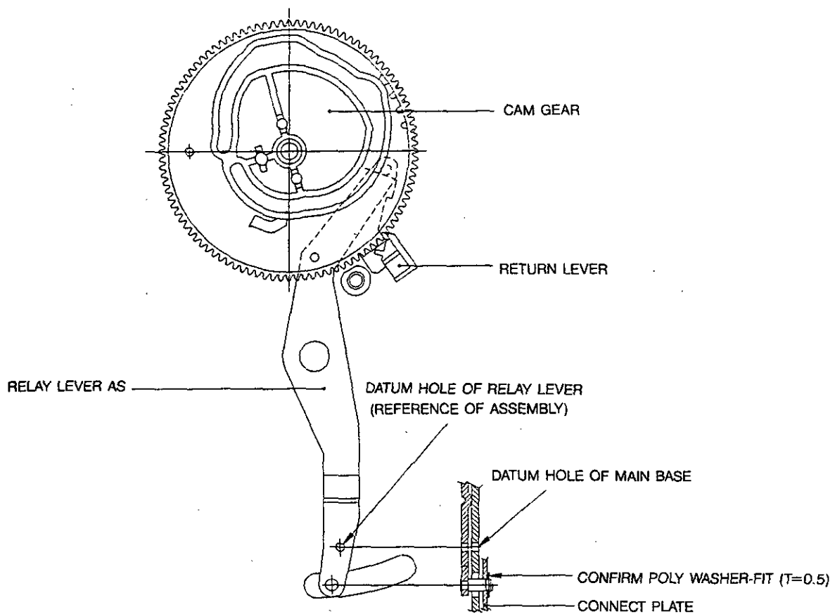
Fig. 4-3 Reference of assembly for the Cam Gear and Relay Lever
