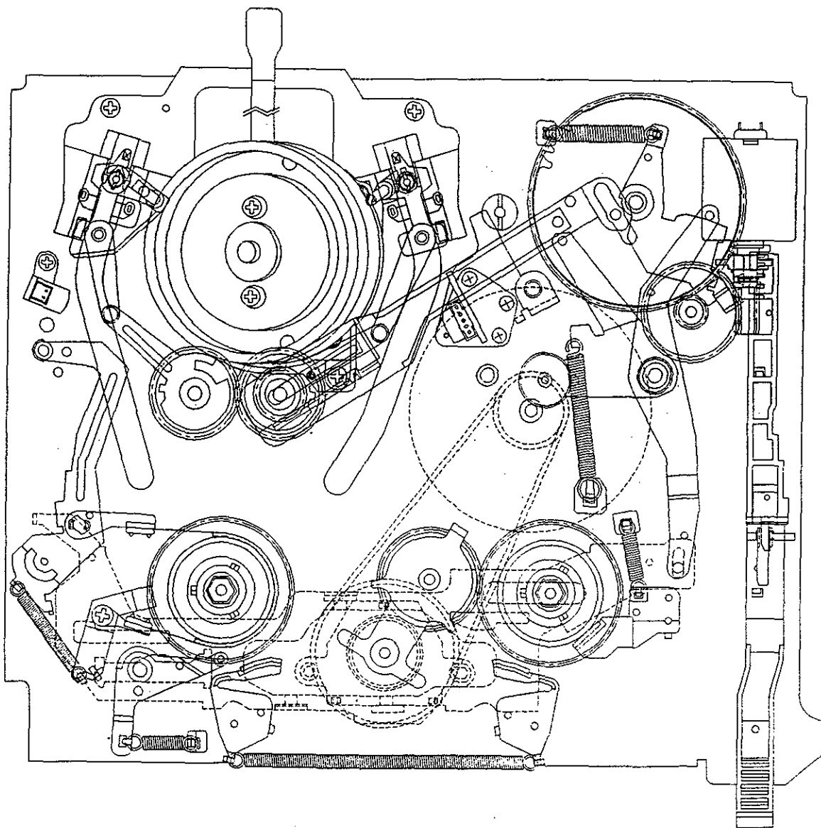
Fig. 1-6. PLAY/RECORD MODE
