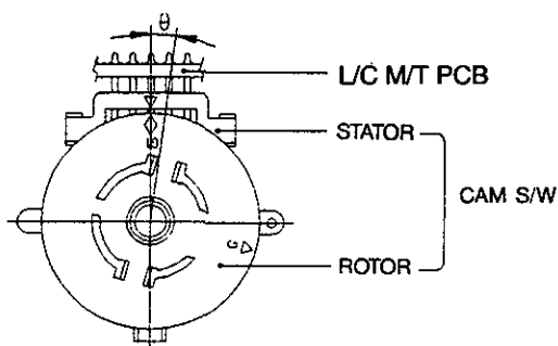
Fig. 4-6 Reference of assembly for the Cam Switch
