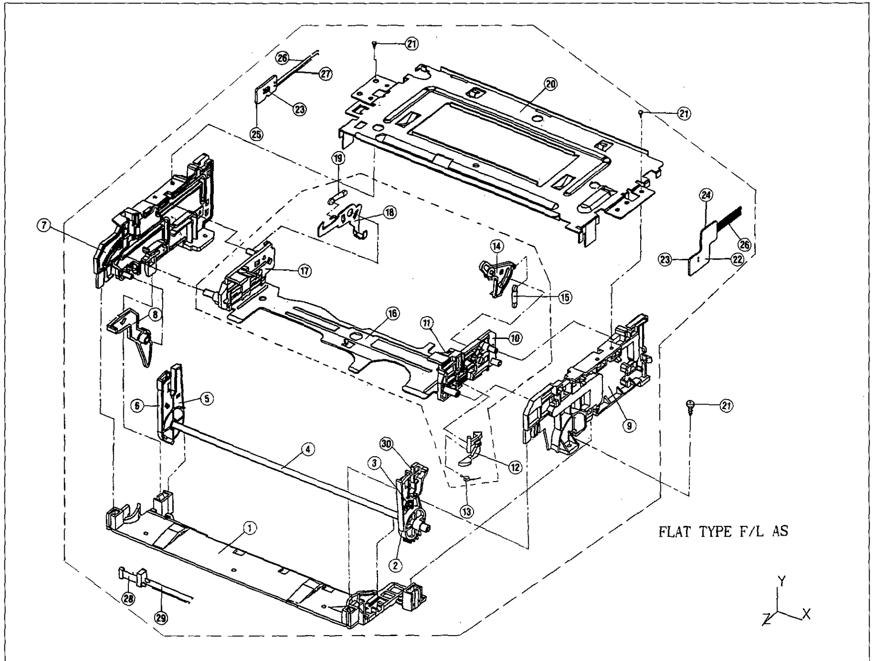
6-3. EXPLODED VIEW OF FRONT LOADING ASS'Y
