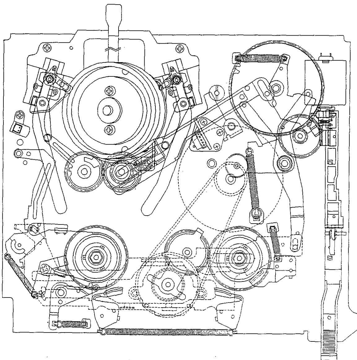
Fig. 1-6. PLAY/RECORD MODE
