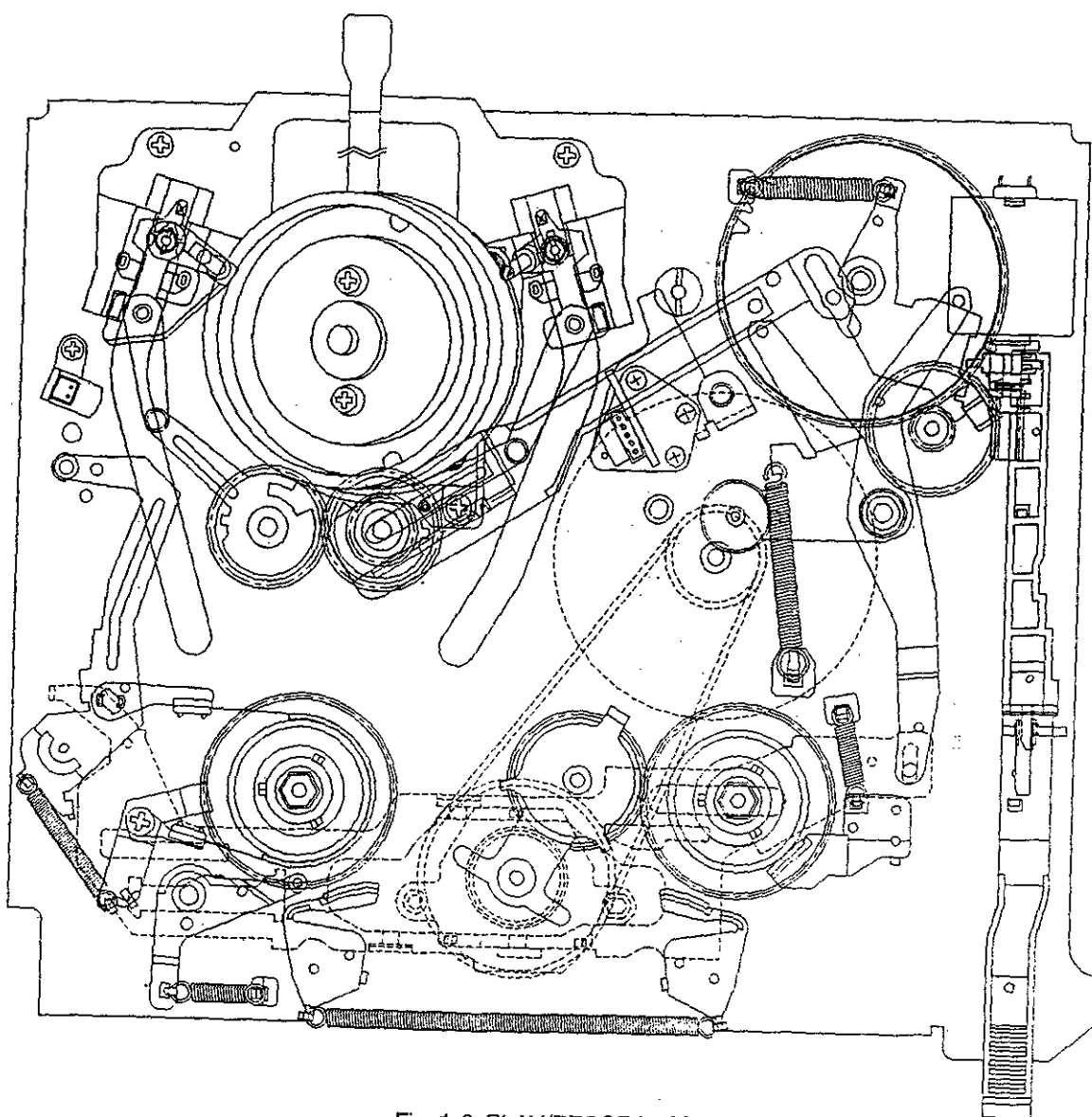
Fig. 1-6. PLAY/RECORD MODE
