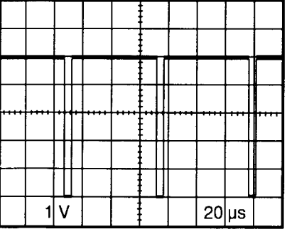
WF19 MAIN 3/4 SCHEMATIC DIAGRAM IC101 PIN 18
