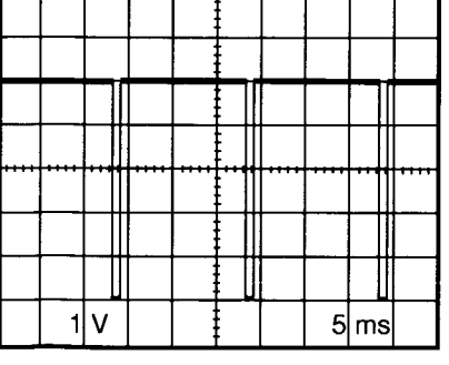
WF20 MAIN 3/4 SCHEMATIC DIAGRAM IC101 PIN 19
