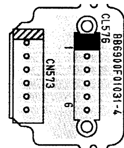
Junction A CBA Top View
