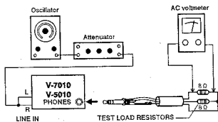
Fig. 3-10 Test setup for PHONES check
