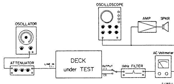
Fig. 8-14 Test Connections for Channel Separation Check
