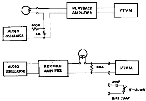
FIG. 10 AMPLIFIER MEASUREMENT
