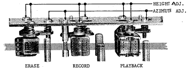
Fig. 5-2 Head Alignment And Adjustment Screws
