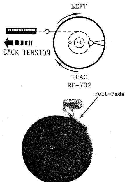
Fig. 6-4 Back Tension Measurement and Adjustment
