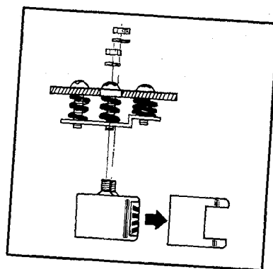
Fig. 5-1 Head Replacement
