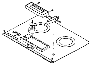
Fig. 4-2 Face Plate Removal
