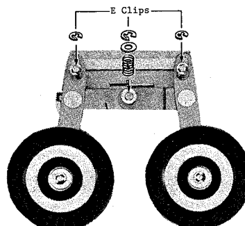
Fig. 4-5 Idlers Removal
