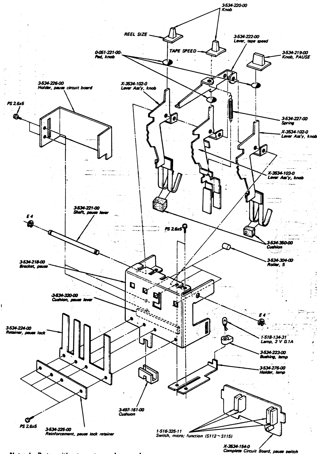
4-5. EXPLODED VIEW (5)
