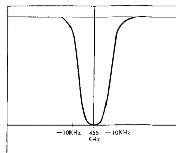
AM IF CHARACTERISTIC
