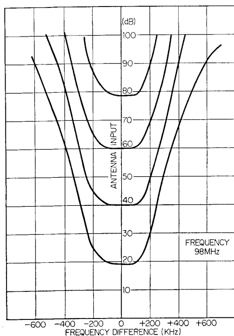
FM SELECTIVITY
