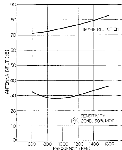
AM SENSITIVITY & IMAGE REJECTION
