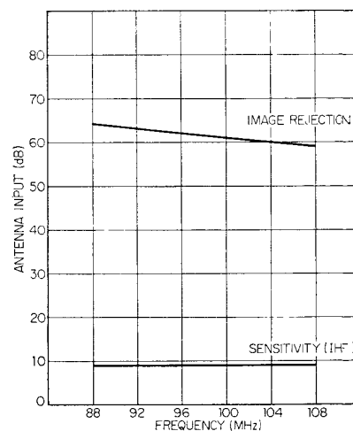
FM SENSITIVITY & IMAGE REJECTION
