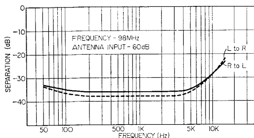
FM MPX SEPARATION
