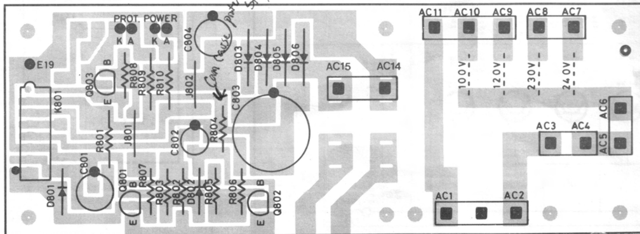
X-1176-01 PCB
