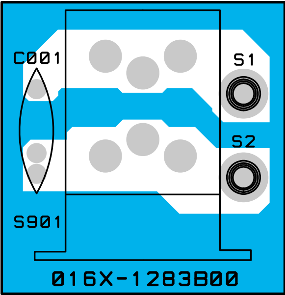
Power Switch PCB 016 X-1283B00
