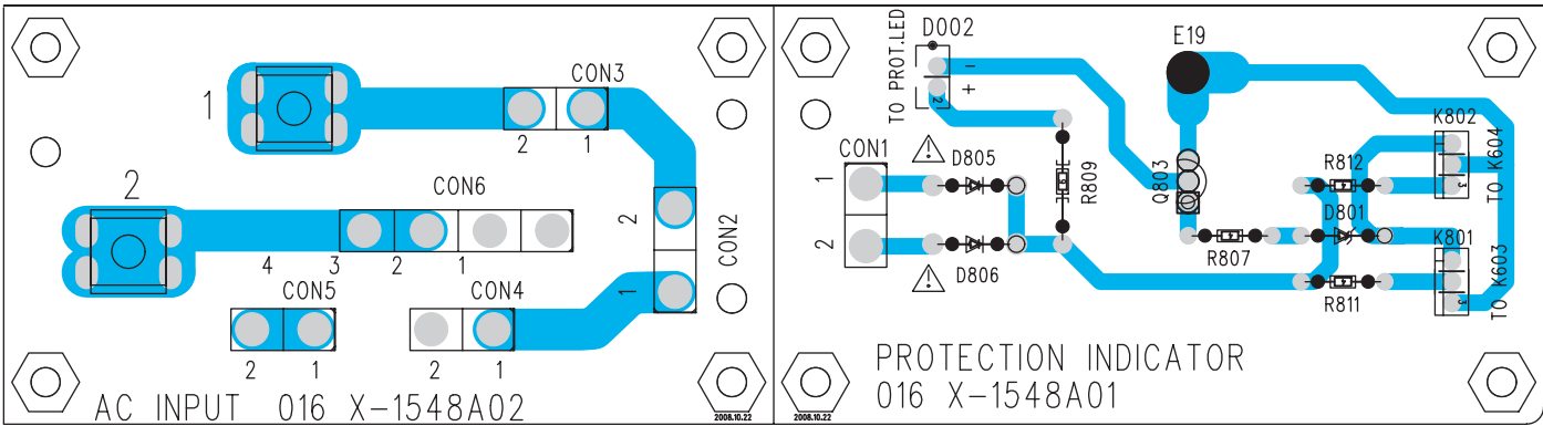
AC INPUT PCB 016 X-1548A01~02
