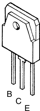
2SA1294 2SC3263
