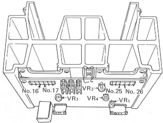
Fig. 10 Power amplifier
