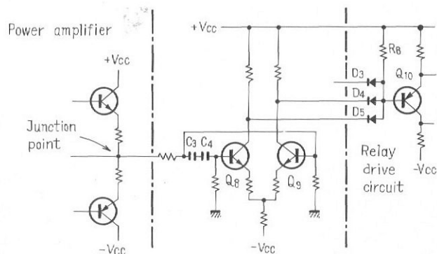
Fig. 7 Center point potential detector
