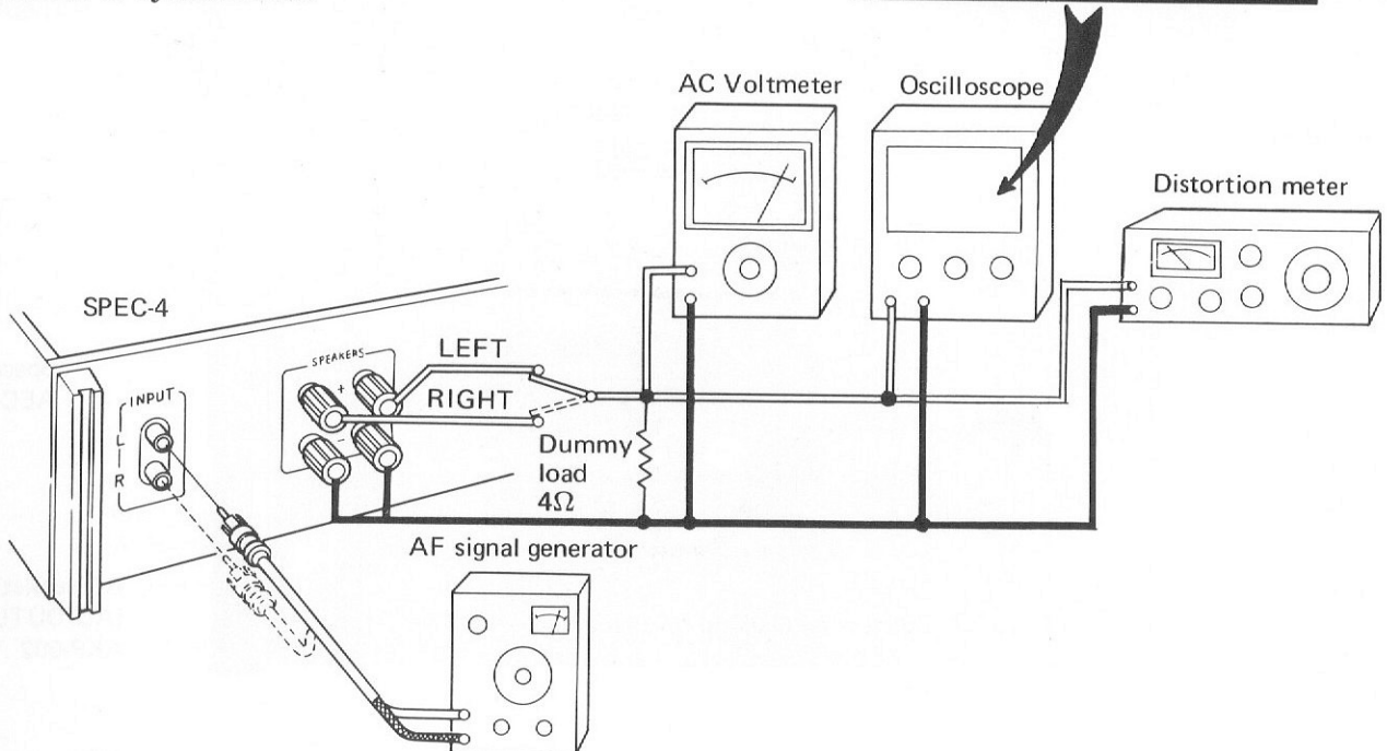
Fig. 11 Connection diagram for power limiter adjustment
