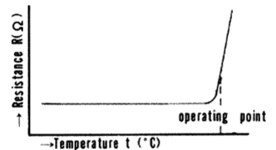
Fig. 8 Posistor-temperature Response
