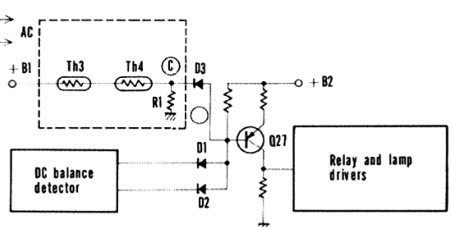
Fig. 9 Temperature Detector Circuit
