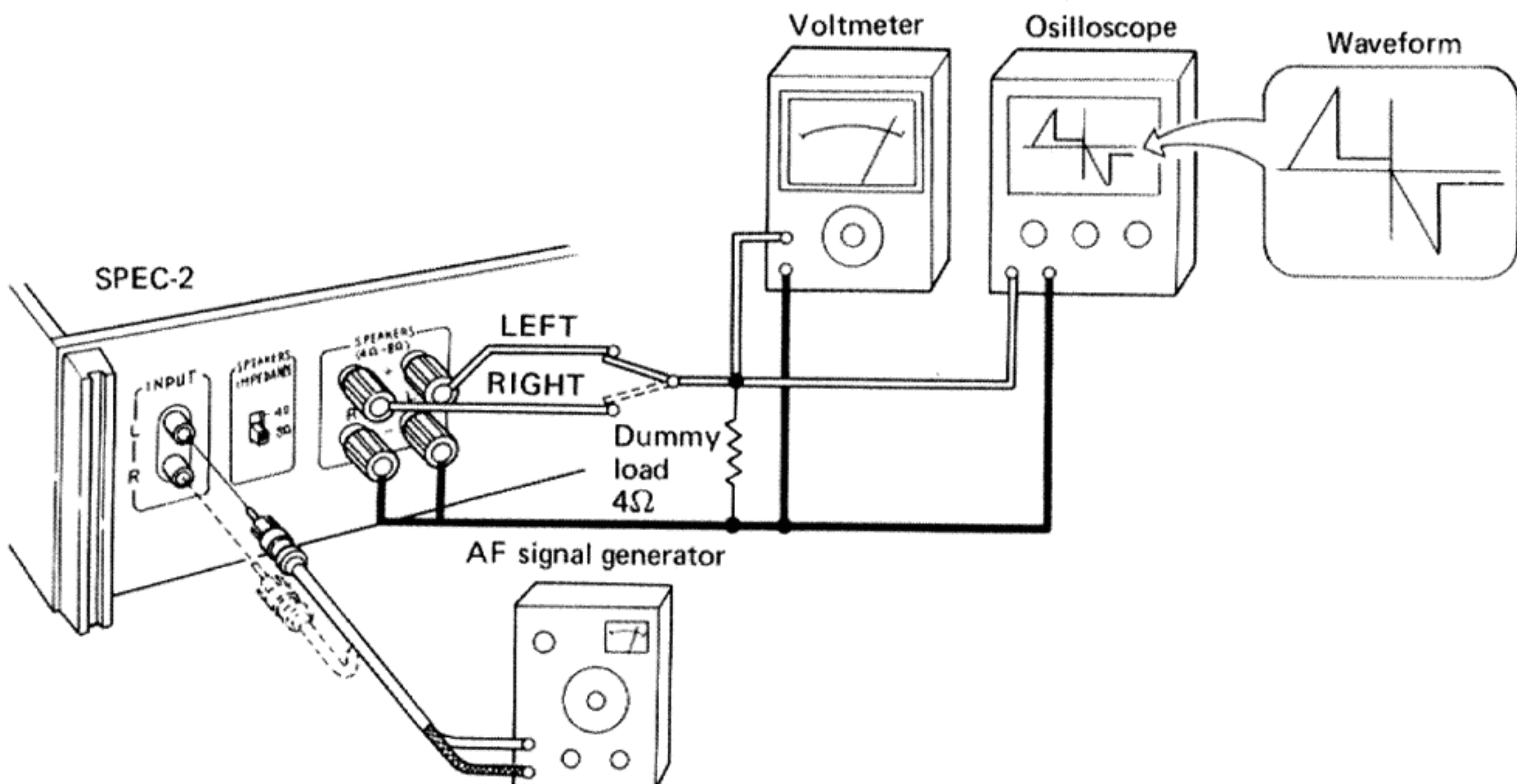
Fig. 14 Connection Diagram for Current Limiter Sensitivity Adjustment
