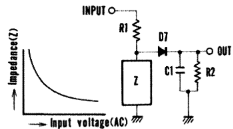
Fig. 4 Equivalent Circuit of the Logarithmic Compression
