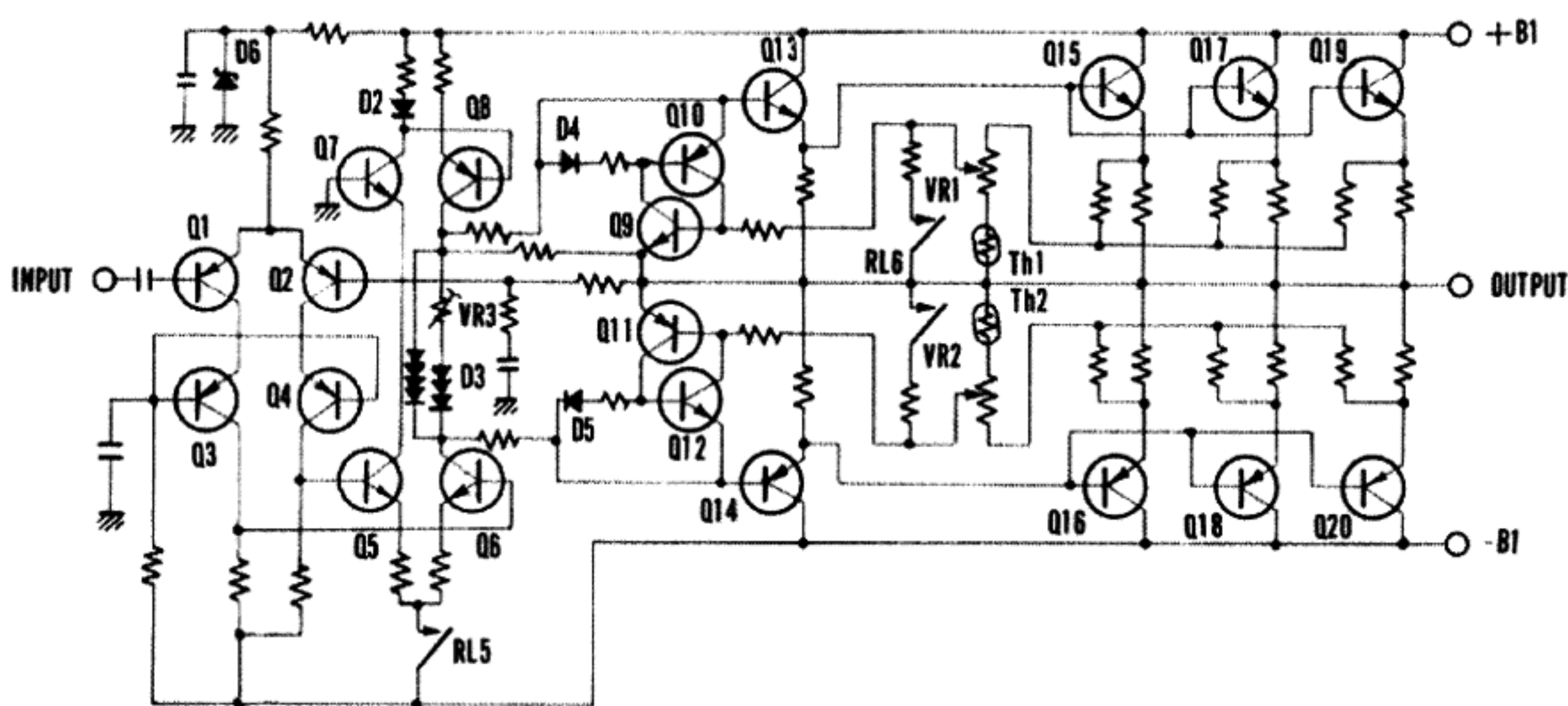
Fig. 2 Power Amplifier Circuit
