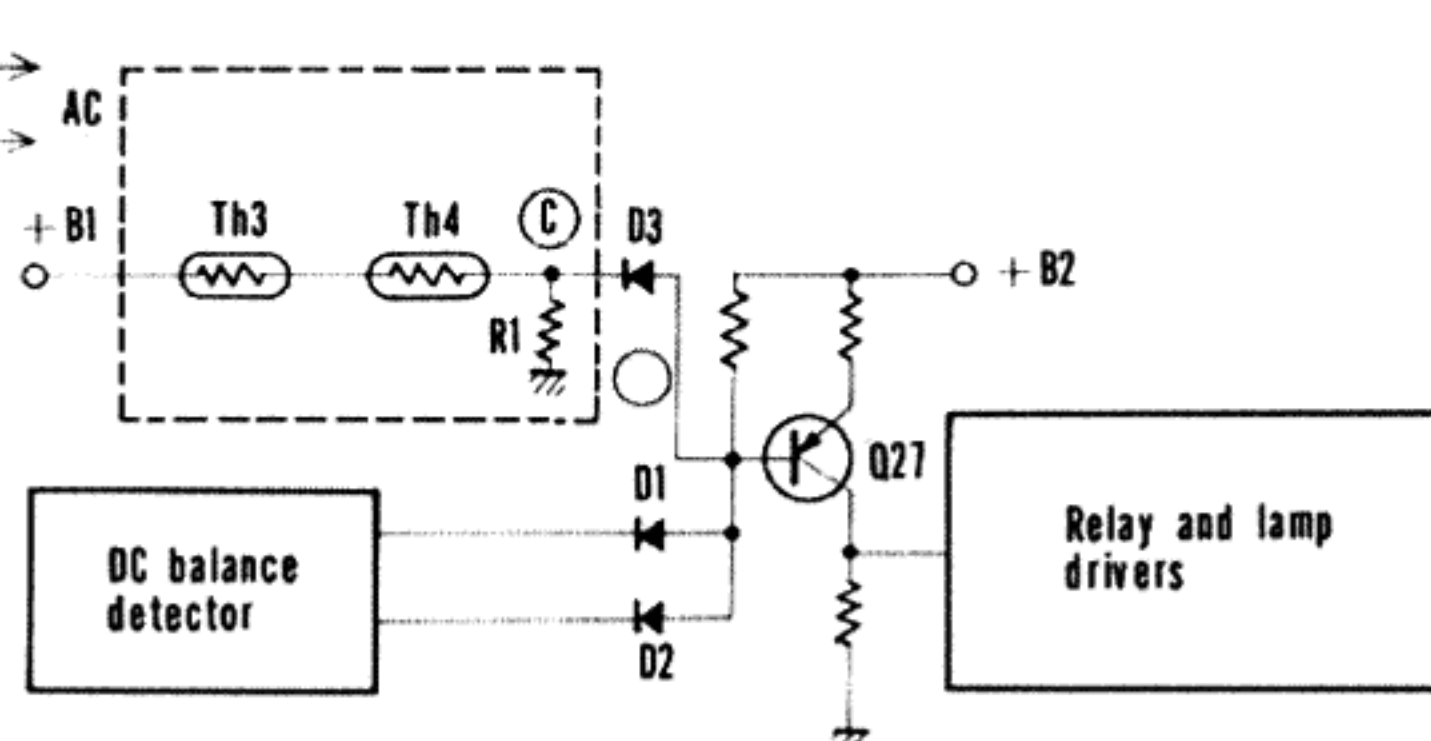
Fig. 9 Temperature Detector Circuit
