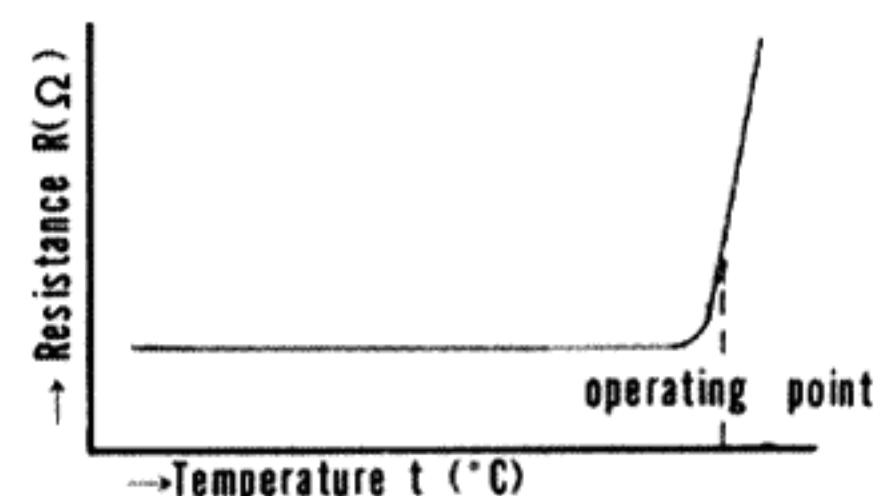
Fig. 8 Posistor-temperature Response
