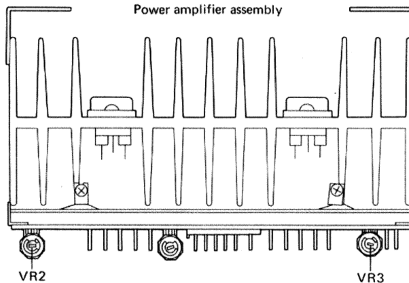
Fig. 13 The Position of VR2 and VR3
