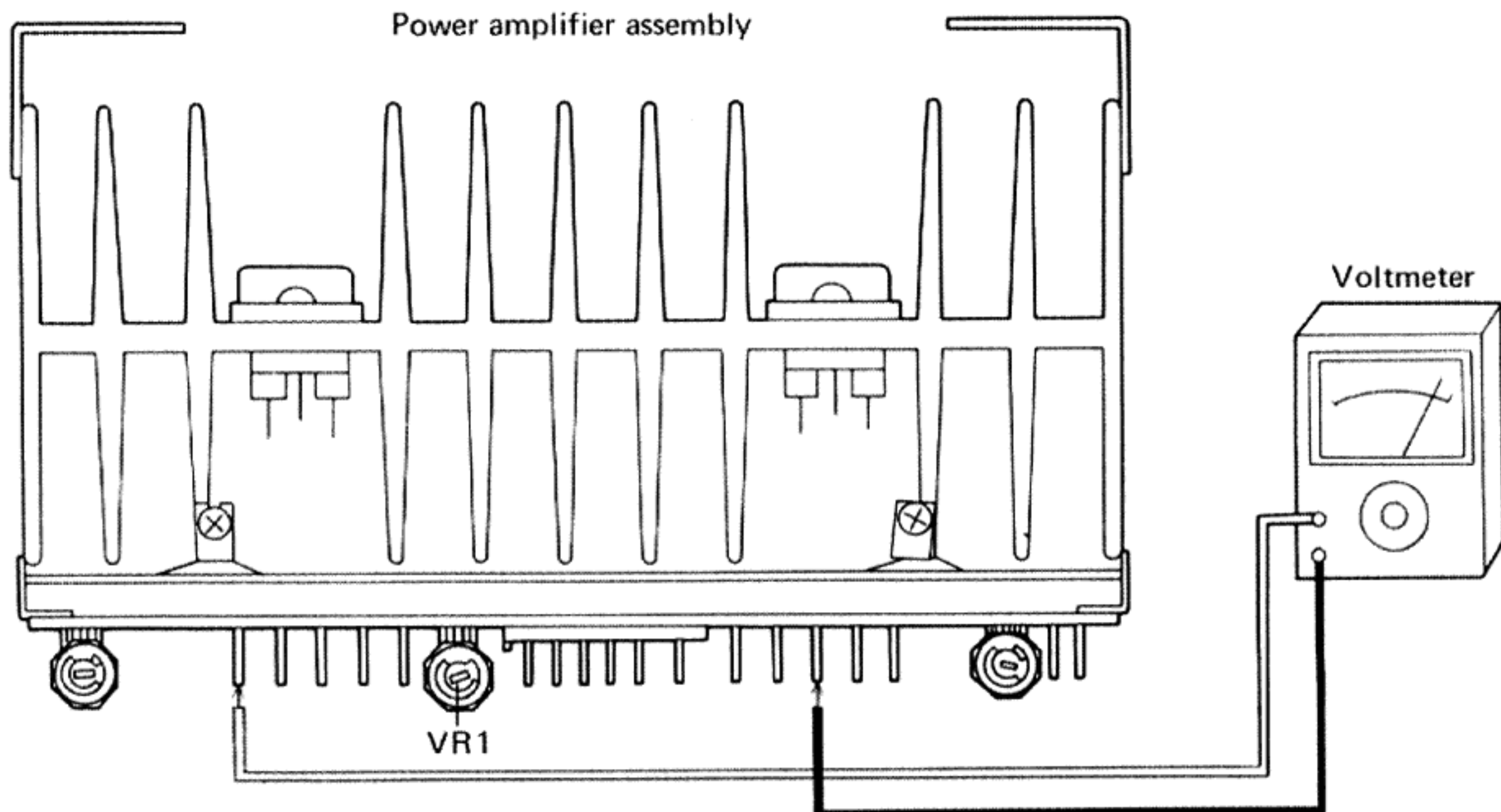
Fig. 12 Connection Diagram for Idle Current Adjustment
