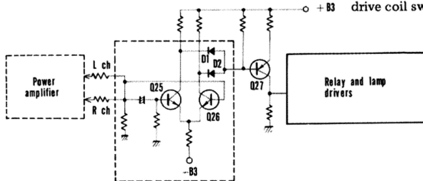
Fig. 10 DC Balance Detector Circuit
