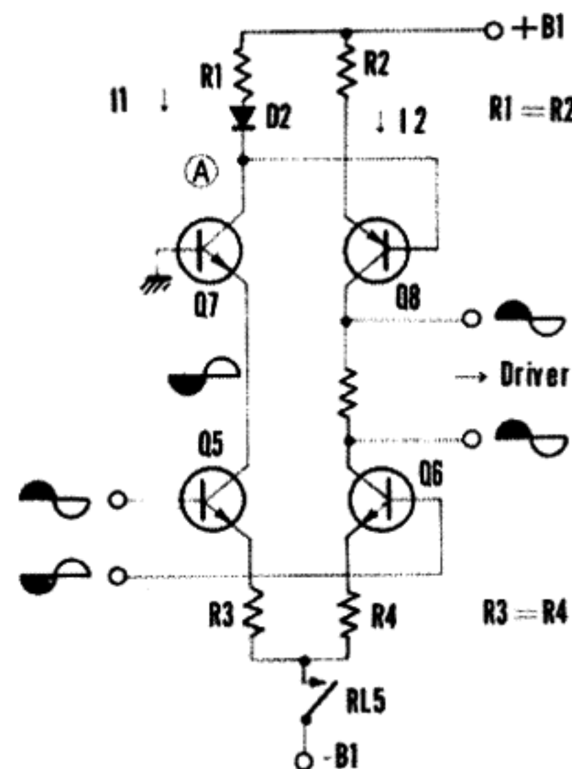
Fig. 1 Current Mirror Circuit
