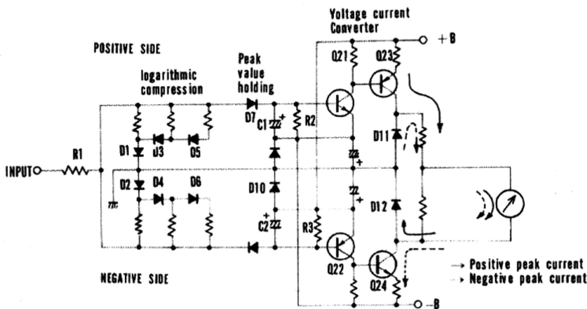
Fig. 3 Peak Level Meter Circuit
