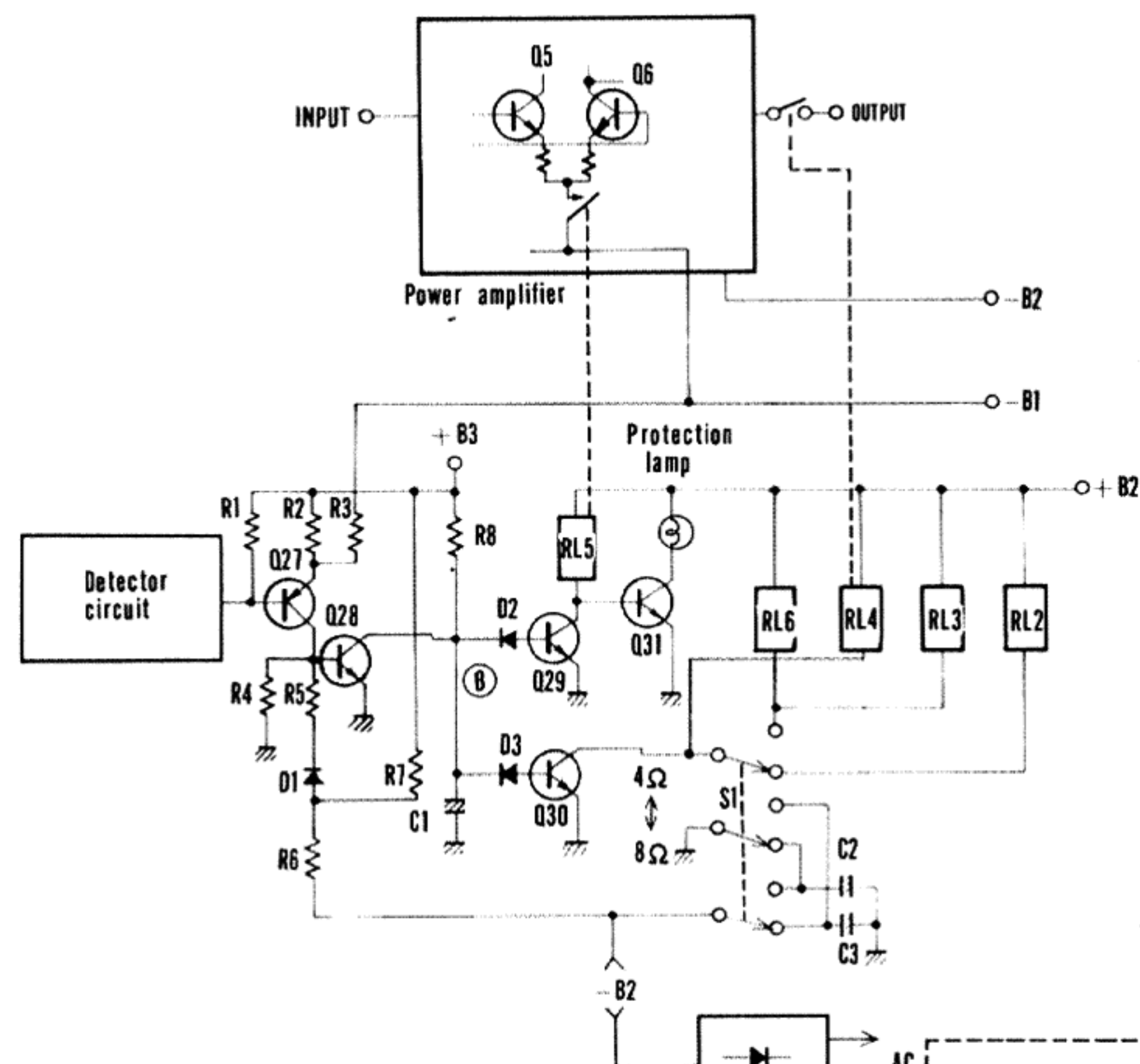
Fig. 7 Relay and Lamp Drivers Circuit
