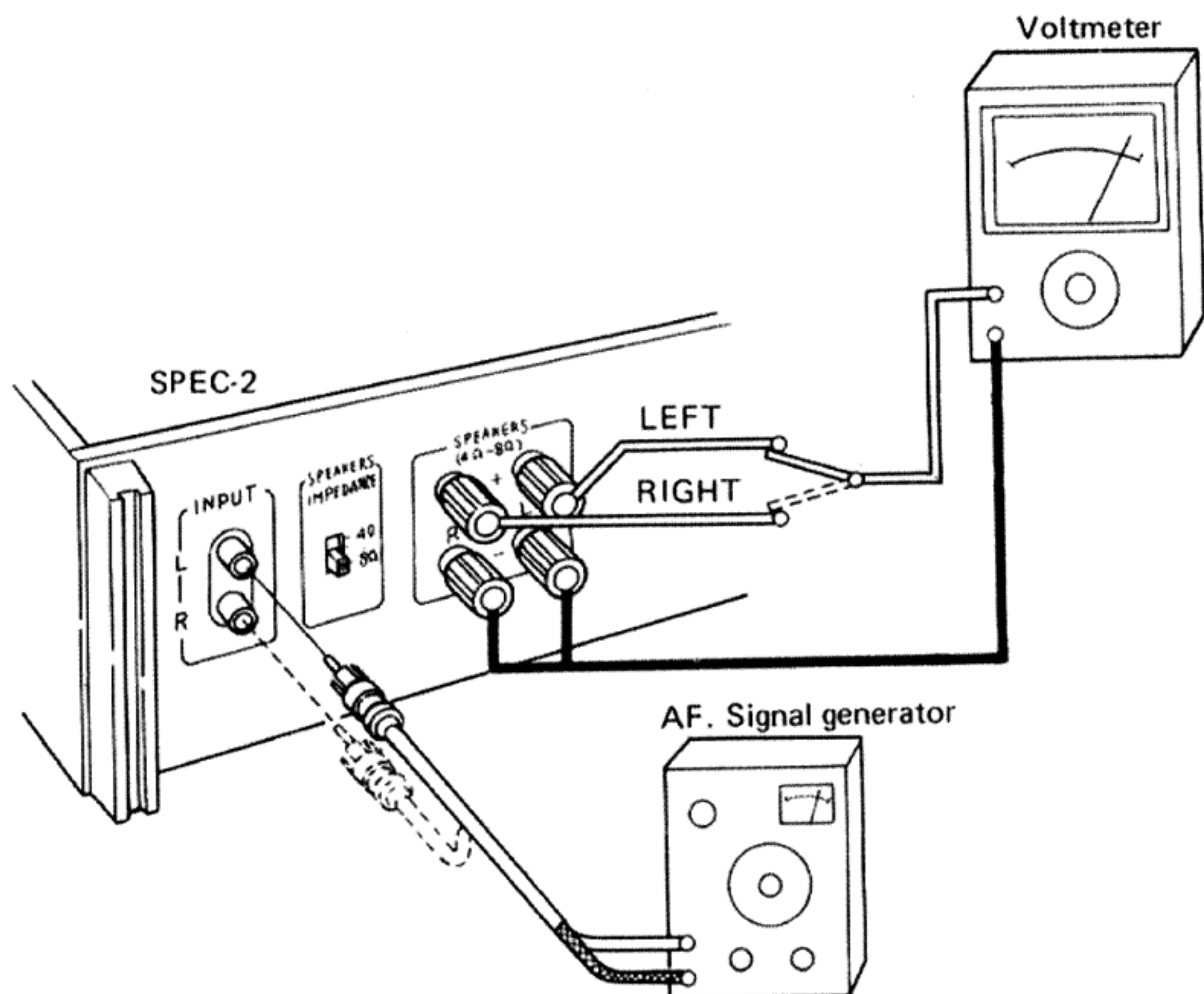
Fig. 16 Connection Diagram for Meter Amplifier Adjustment
