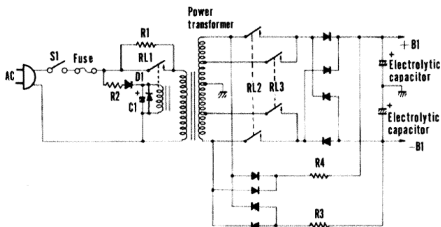
Fig. 11 Surge Current Suppressor Circuit
