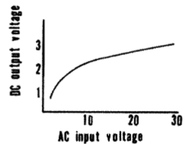
Fig. 5 Input-output Response
