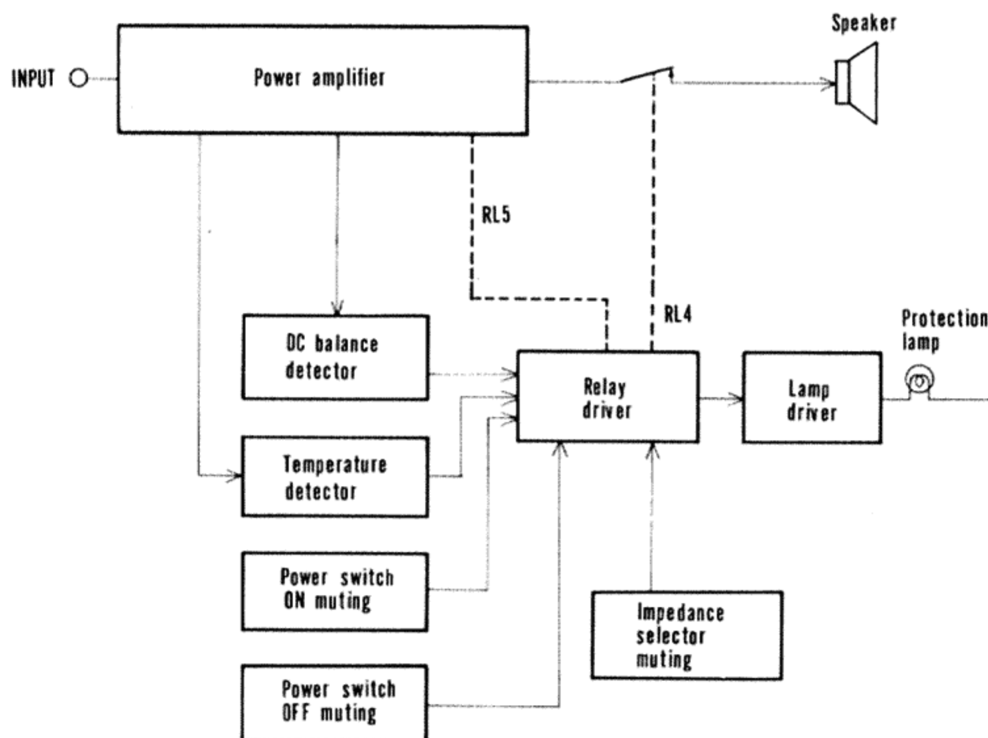
Fig. 6 Block Diagram of the Protection Circuit
