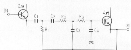
Fig. 7 Circuit Diagram of Filter Circuit
