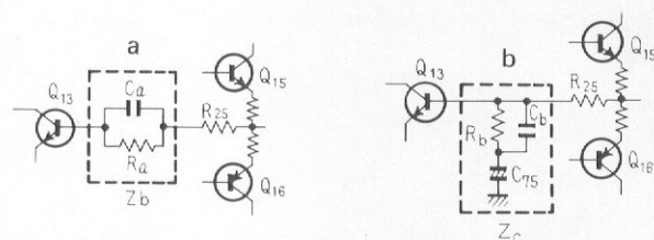
Fig. 8 Equivalent Circuit of Bass Boost and Cut
