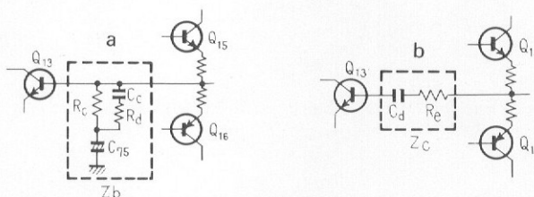
Fig. 9 Equivalent Circuit of Treble Boost and Cut
