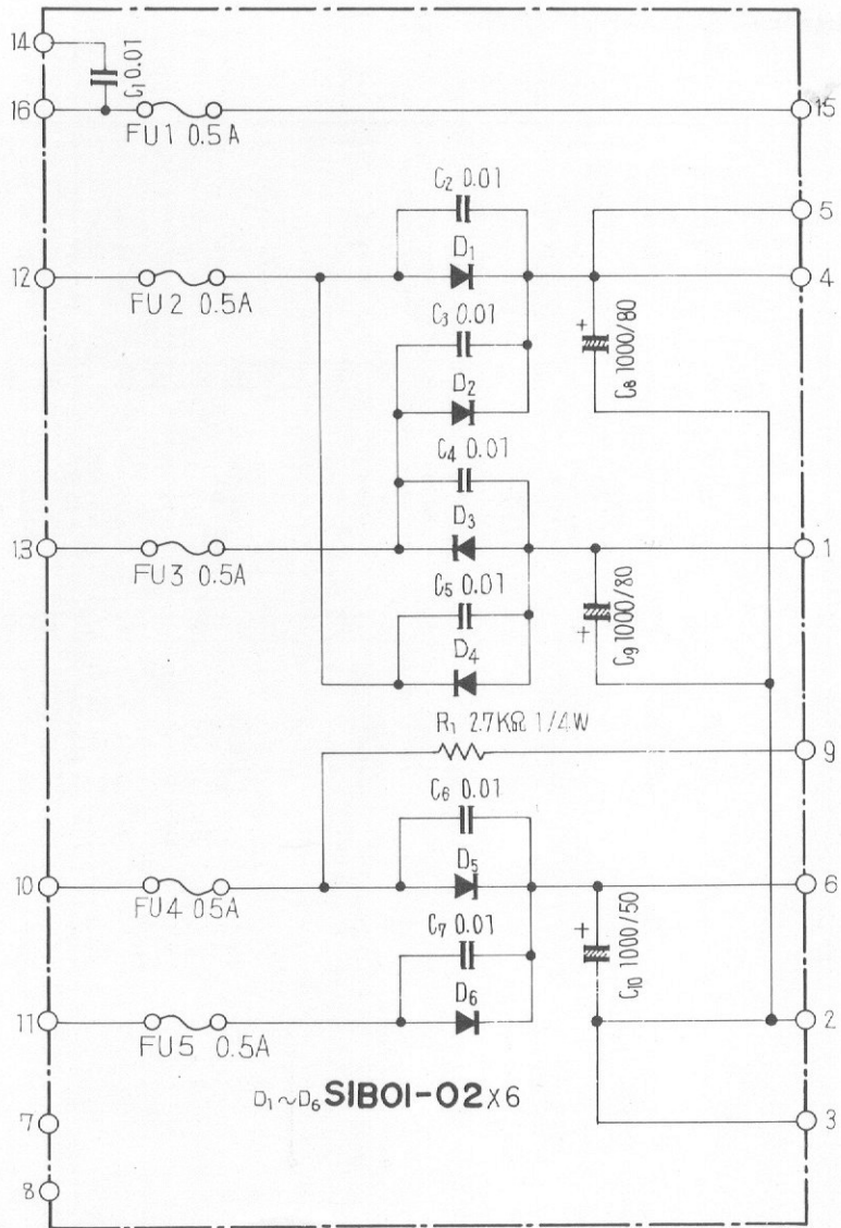
Parts List of Fuse Board Assembly (AWX-091)
