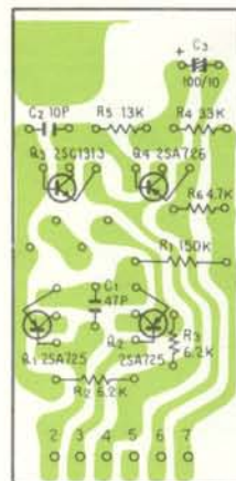
AWK-065 PCB
