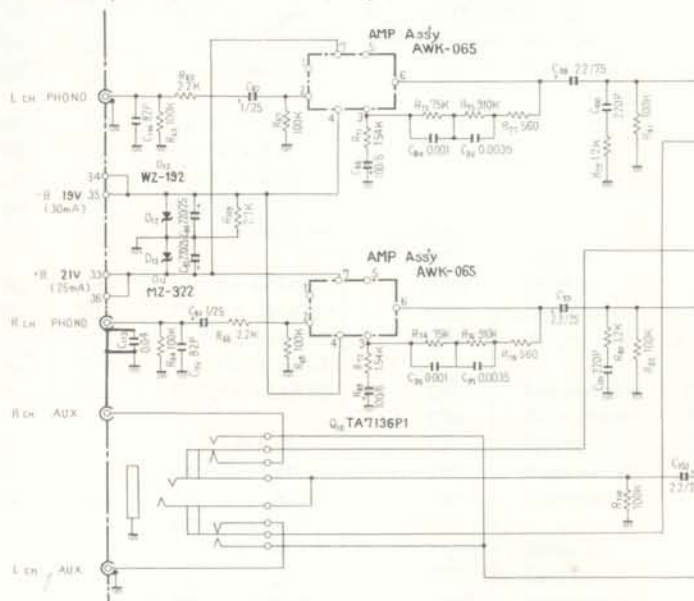
AWK-065 PCB
