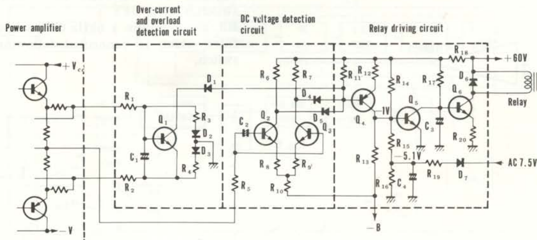
Fig. 9 Protection Circuit
