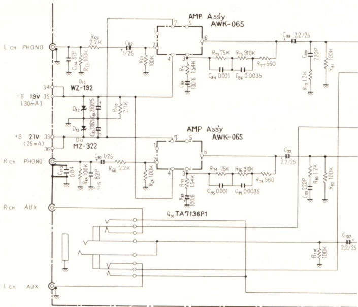
AWK-065 PCB
