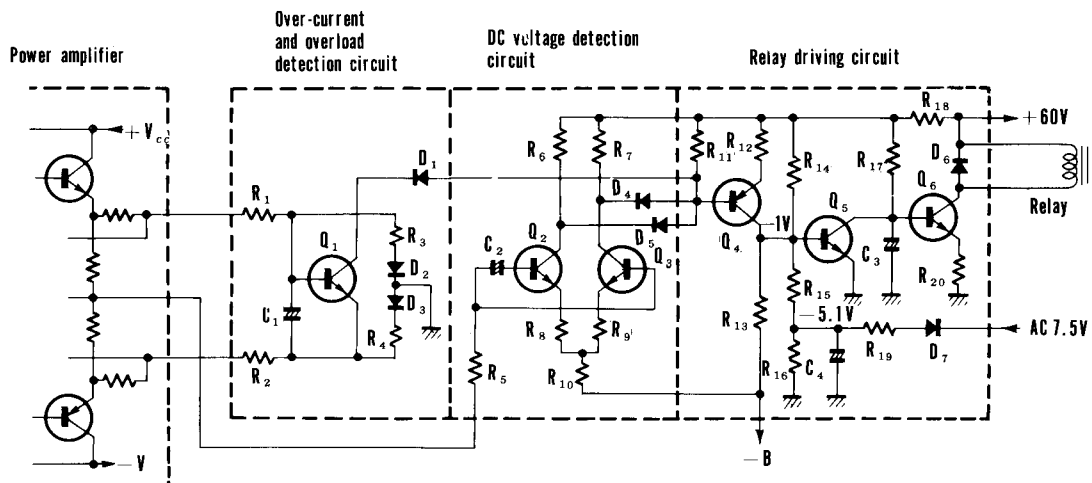
Fig. 9 Protection Circuit
