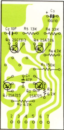
AWK-065 PCB
