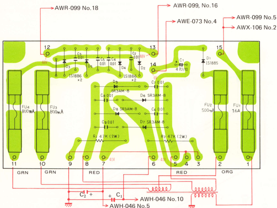
Parts List of Power Supply Assembly (AWR-116)
