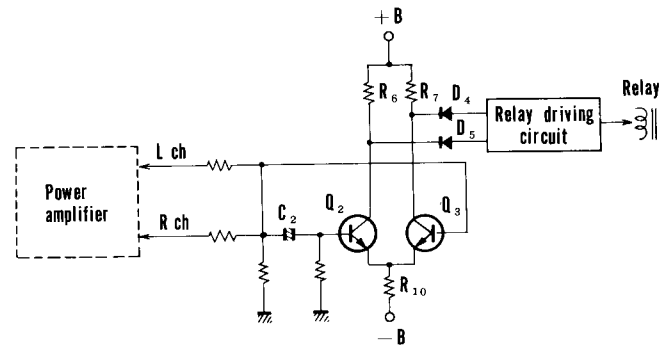
Fig. 10 DC Voltage Detection Circuit
