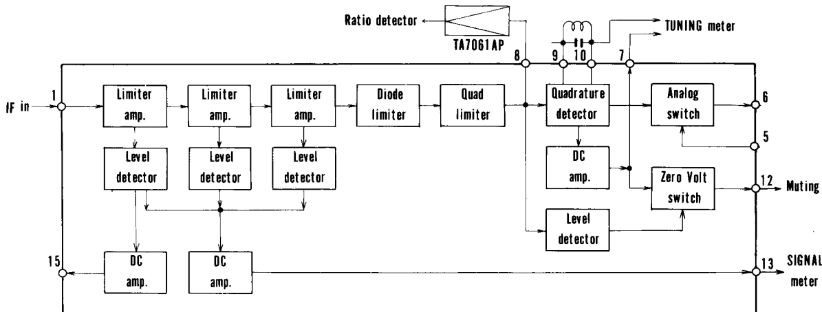
Fig. 2 Block Diagram of HA1137
