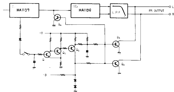
Fig. 5 FM Muting Circuit
