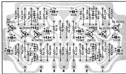
Equalizer amp ass'y AWF-011
