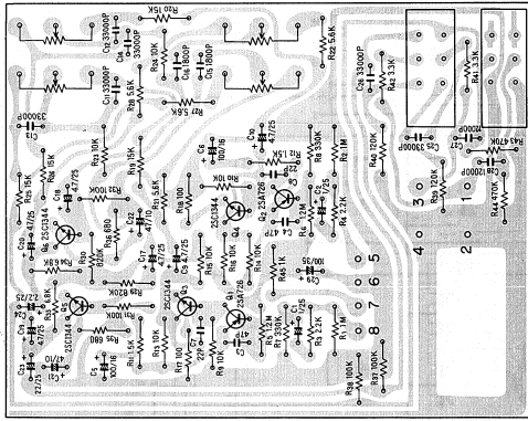
Control amp ass'y AWW-030
