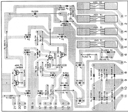
Power supply ass'y AWR-057 (F.KCU model)
