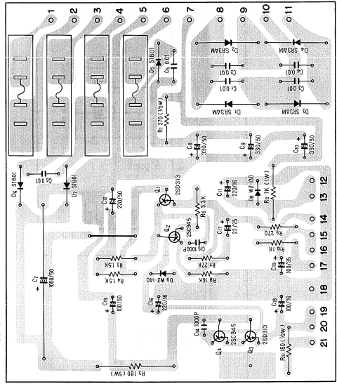
Power supply ass'y AWR-058 (GN model)
