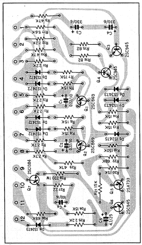
Protection ass'y AWM-025
