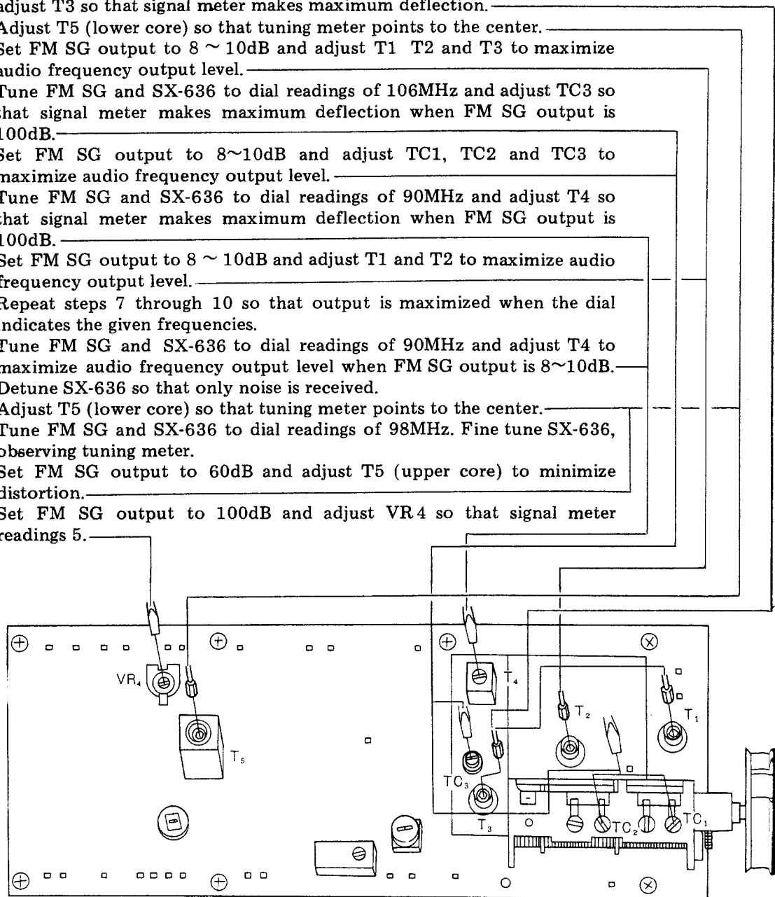
TUNER ASSEMBLY (AWE-04)
