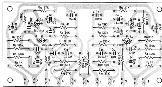
Equalizer amp ass'y W21-004
