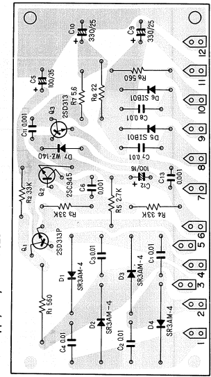
Power supply ass'y AWR-029
