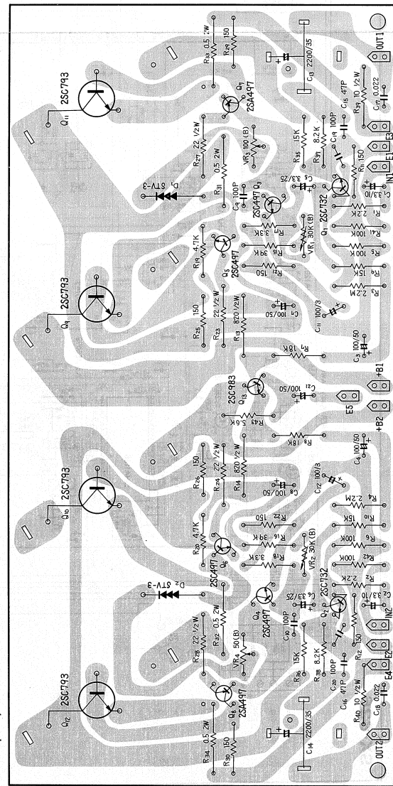
Power amp ass'y AWH-002
