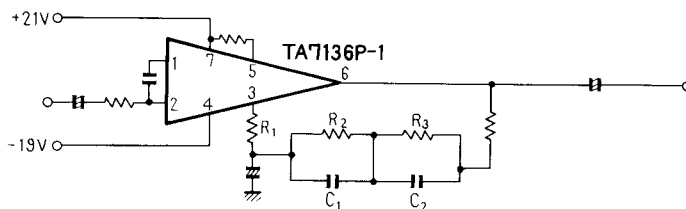
Fig. 2 PHONO Equalizer
