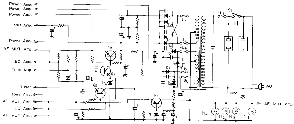
Fig. 8 Power Supply
