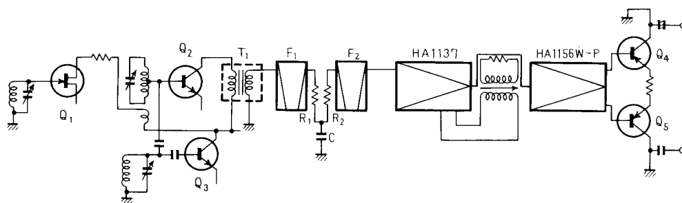
Fig. 1 Tuner Section
