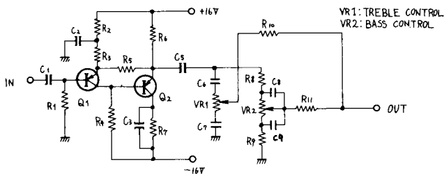
Fig. 4 Tone Control
