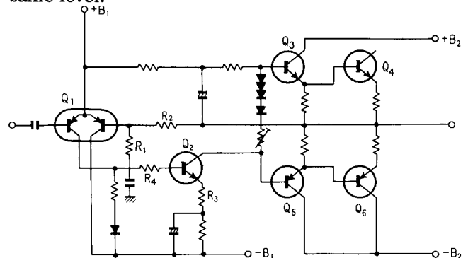
Fig. 7 Power Amplifier
