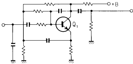
Fig. 3 Microphone Circuit
