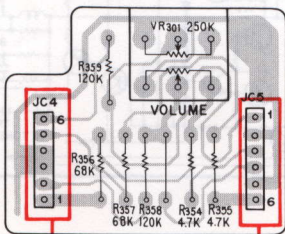
VOLUME Ass'y
