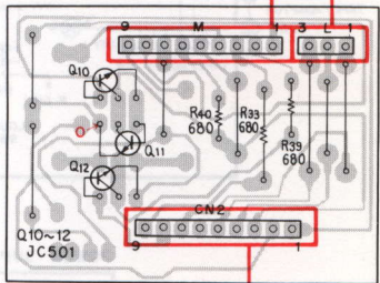
CONTROL Ass'y(A)
