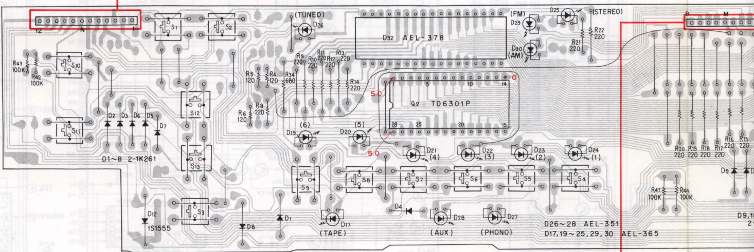
CONTROL Ass'y(GWX-706)
