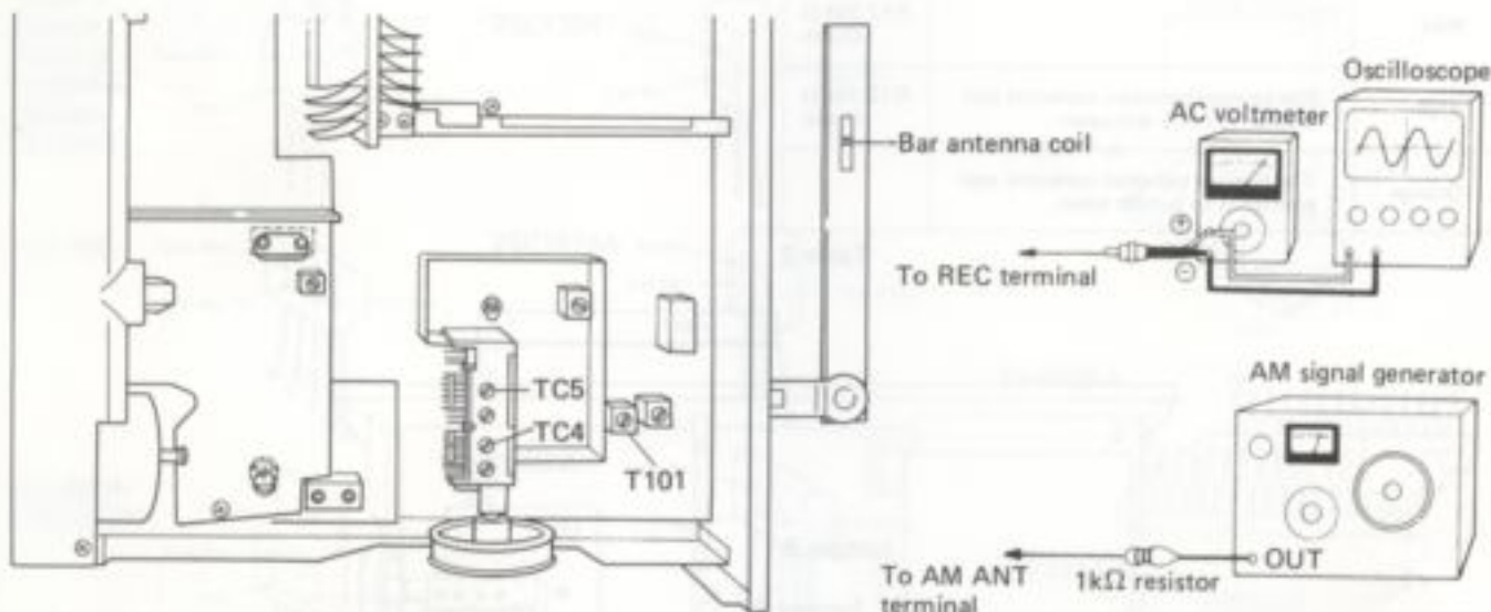
Fig. 8-3 Adjustment point
