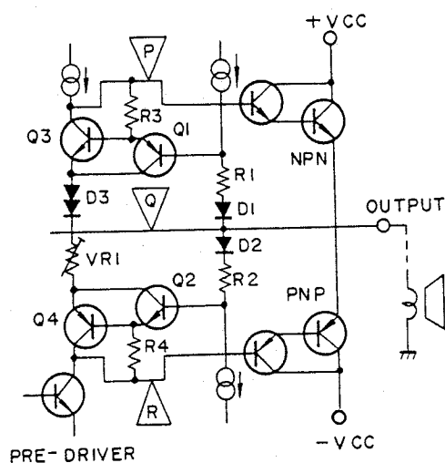
Fig. 5-9 NSA Circuit
