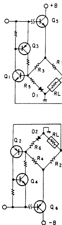
Fig. 5-7 Bridge Circuit
