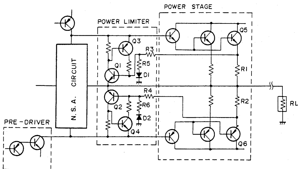
Fig. 5-6 Power Limiter
