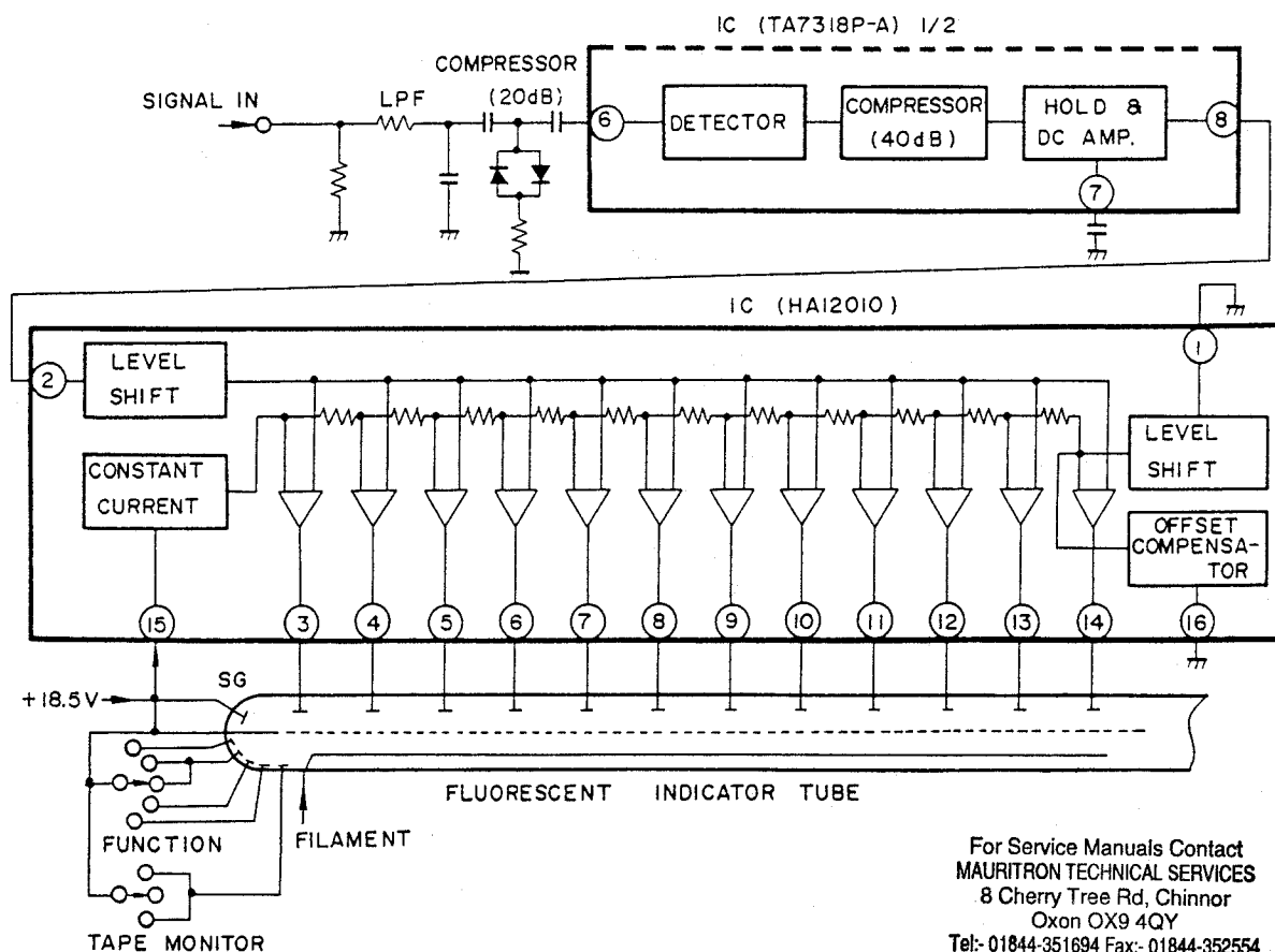
Fig. 5-12 Indicator Circuit
