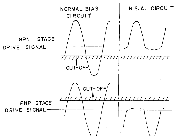
Fig. 5-11 Driving Signal of Power Stage
