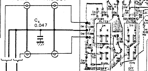
FILTER ASS'Y (GWS-1)
