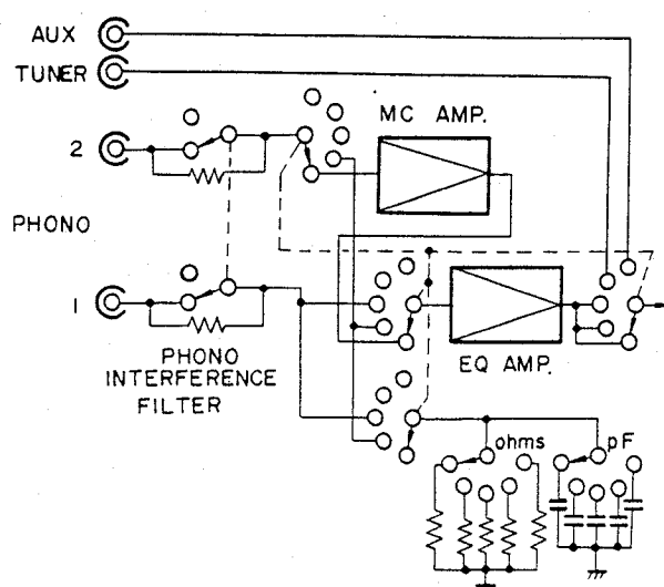
Fig. 5-1 Phono Circuit
