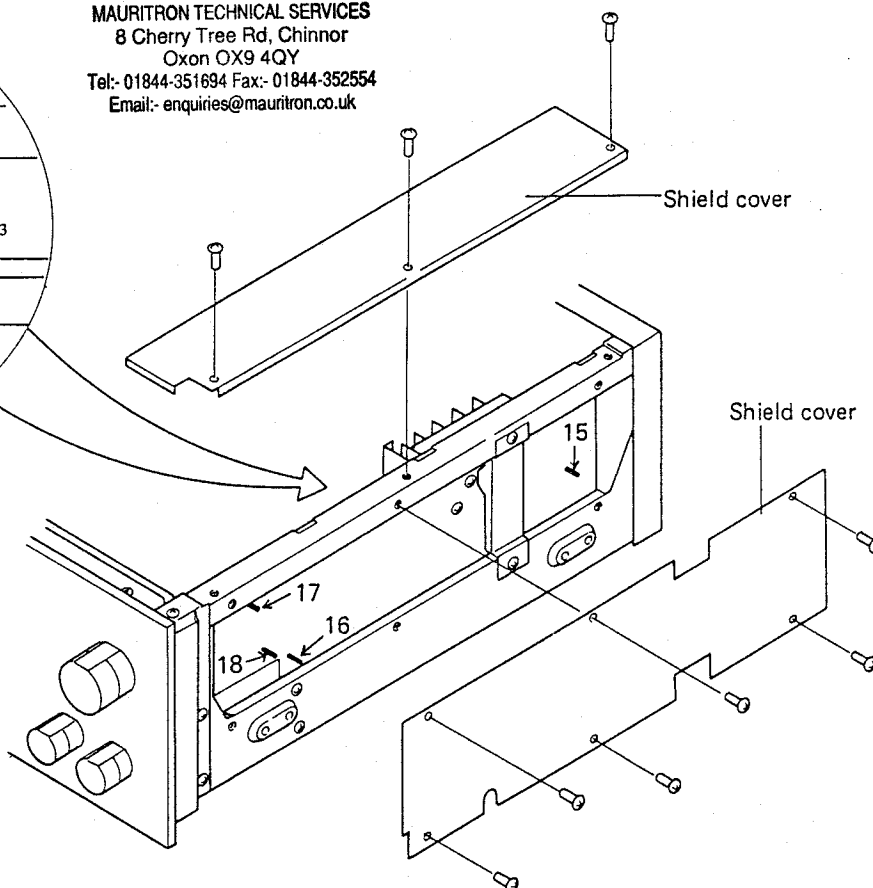
Fig. 8-3 Adjustments of Preamplifier
