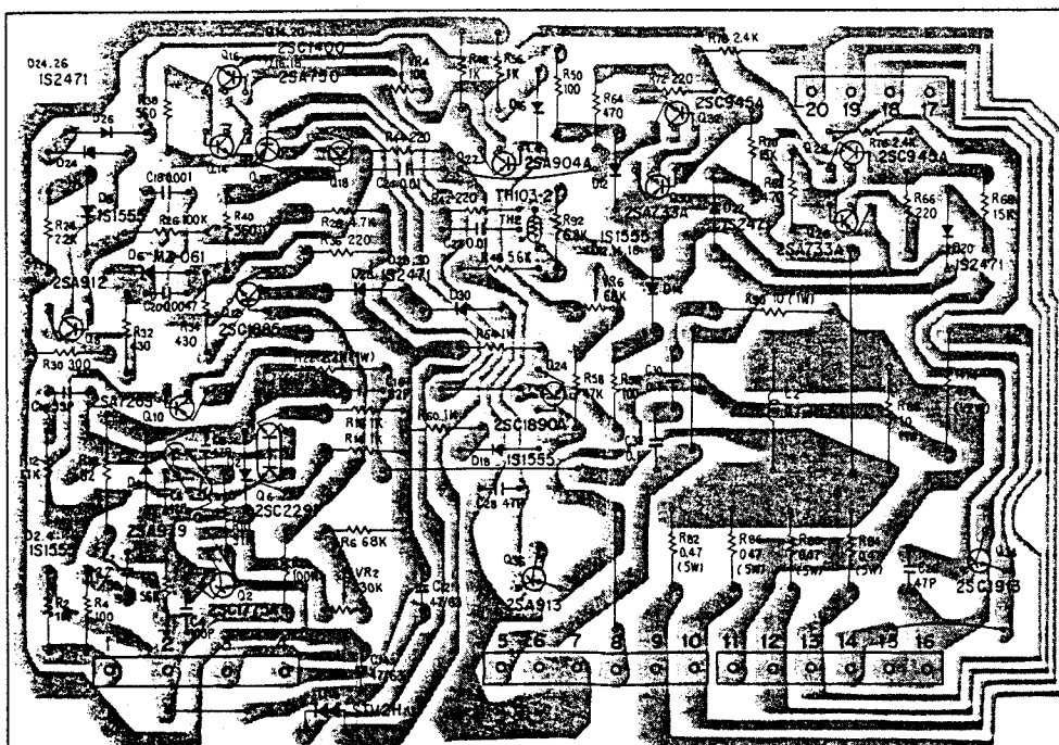
PA-R Assembly (GWH-126)
