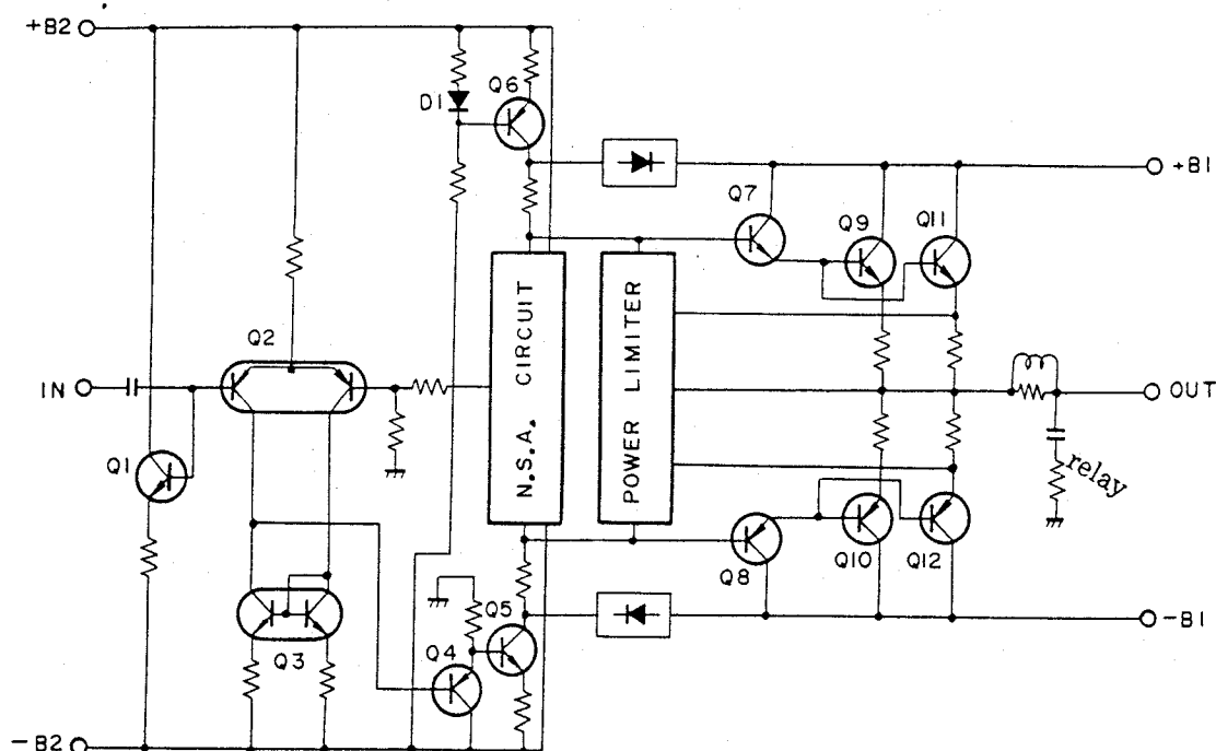
Fig. 5-5 Power Amplifier
