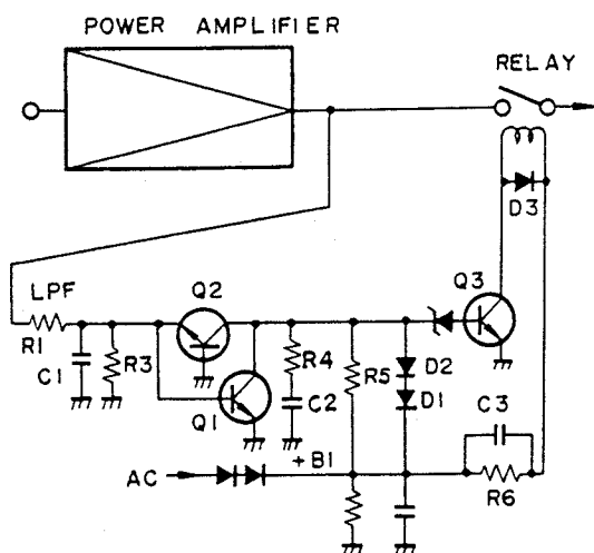
Fig. 5-13 Protection Circuit
