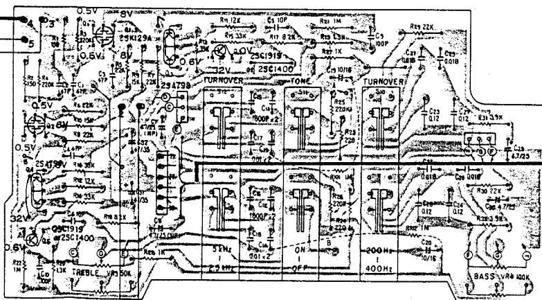
TC ASS'Y (GWG-124)
