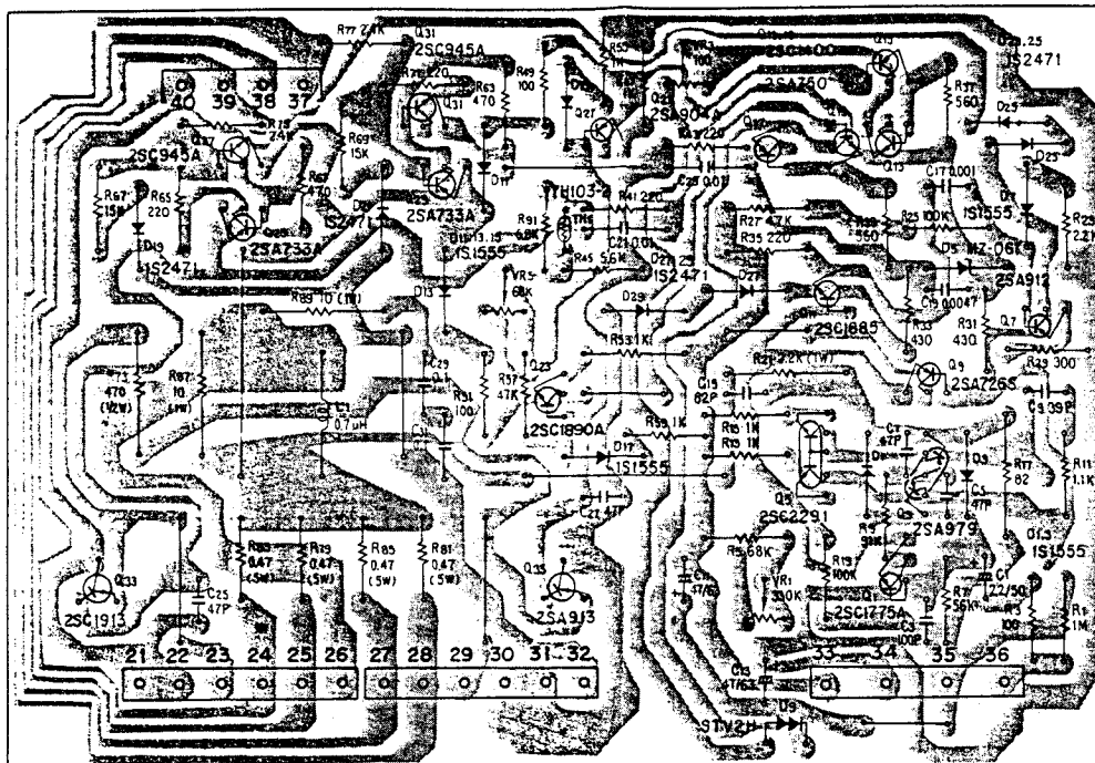
PA-L Assembly (GWH-125)
