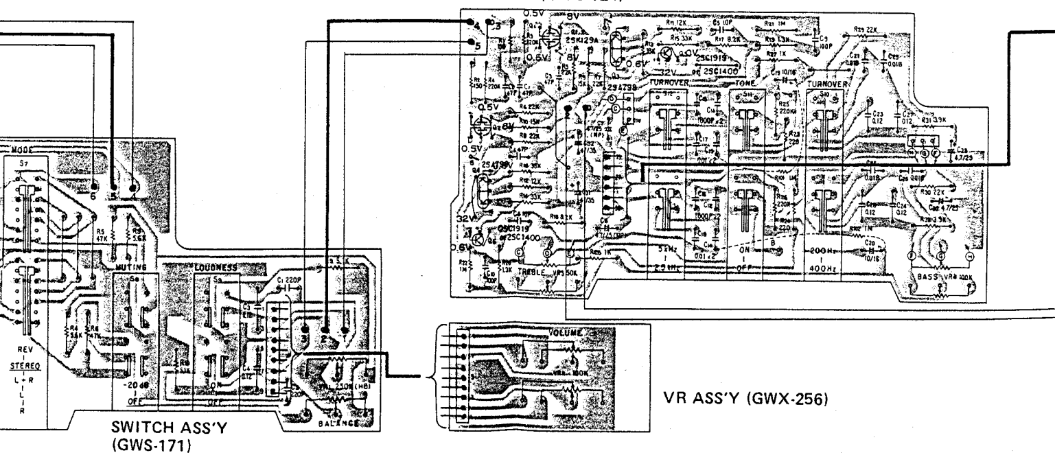
TC ASS'Y (GWG-124)
