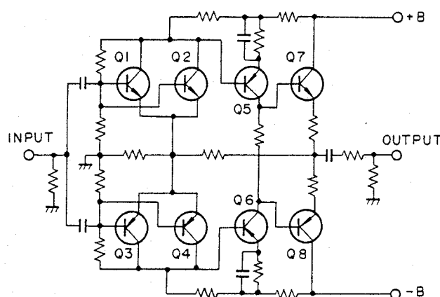
Fig. 5-2 MC Amplifier
