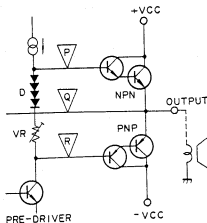
Fig. 5-8 Normal Power Stage
