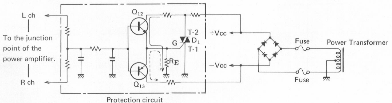
Fig. 2 Protection circuit
