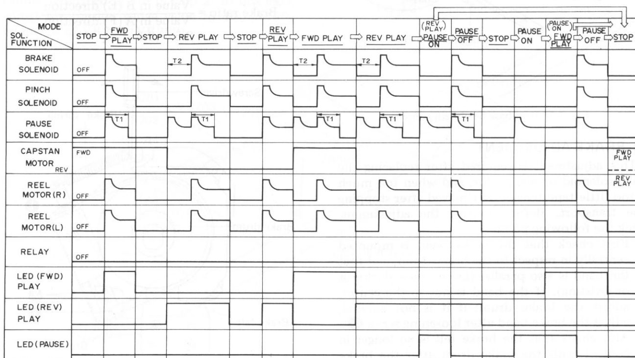
Fig. 6-8 Timing chart
