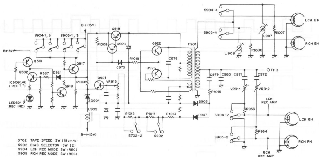
Fig. 6-1 Oscillator circuit
