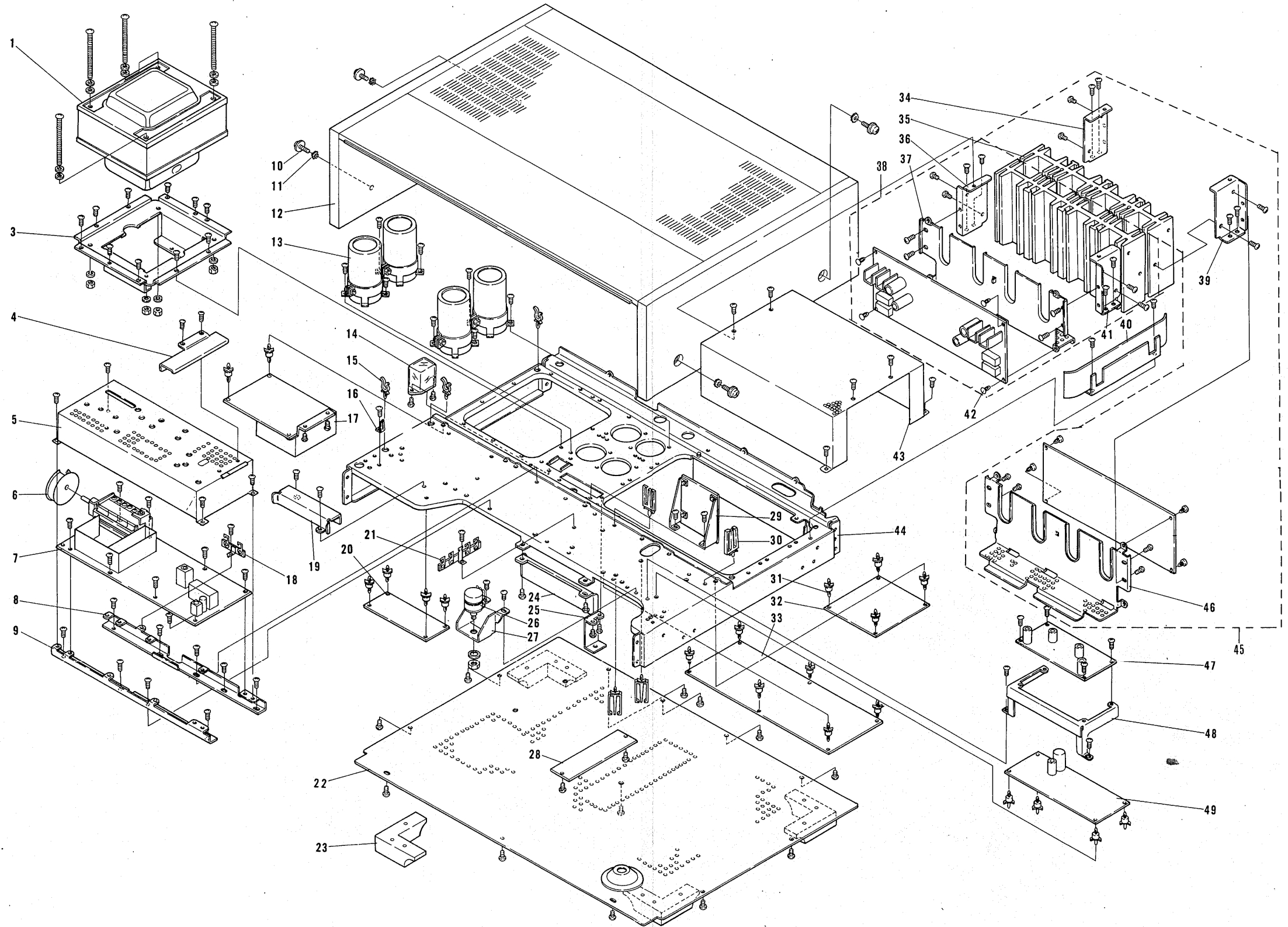
EXPLODED VIEW-1
