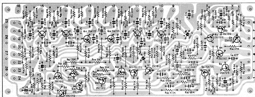
Decoder ass'y AWM-031
