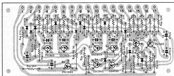
Protection circuit ass'y AWM-049
