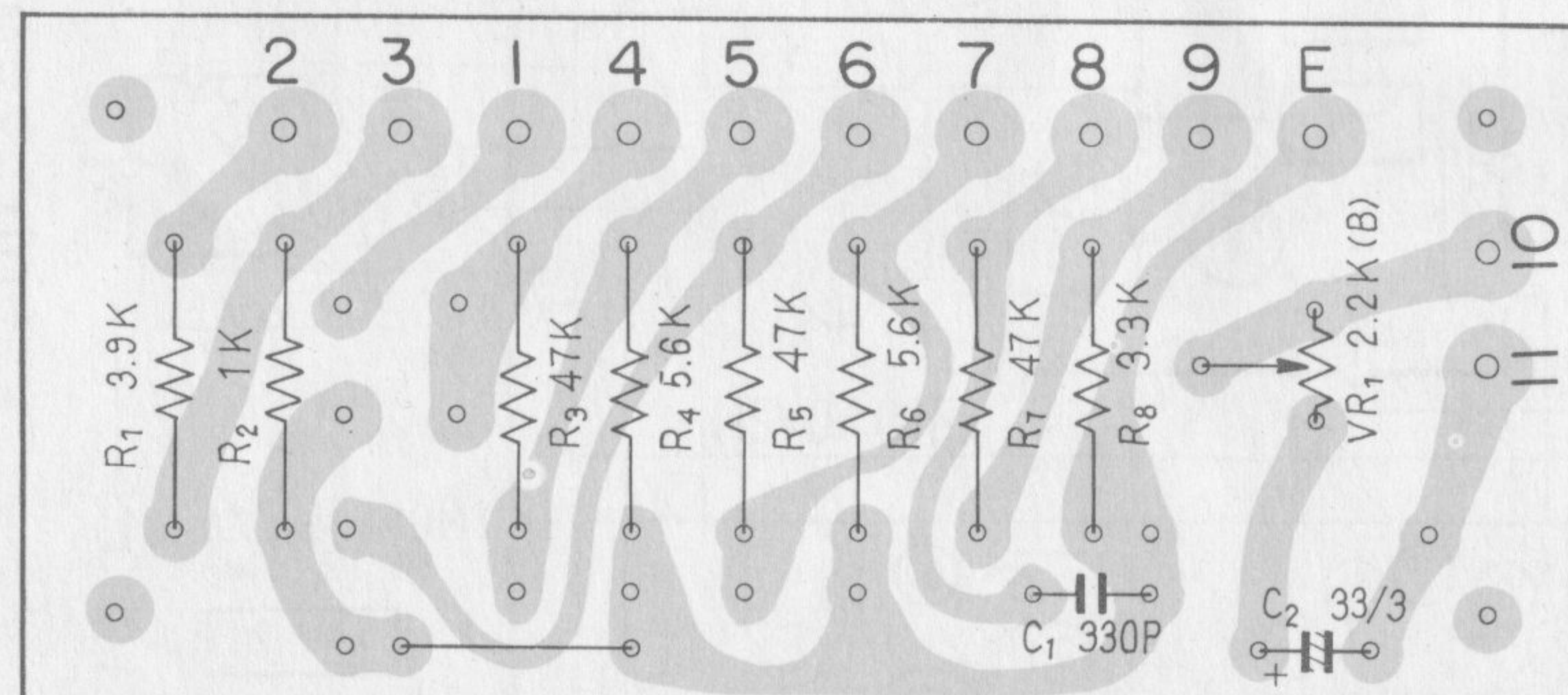
CR ass'y AWE-012 (FSAW, FW model)
