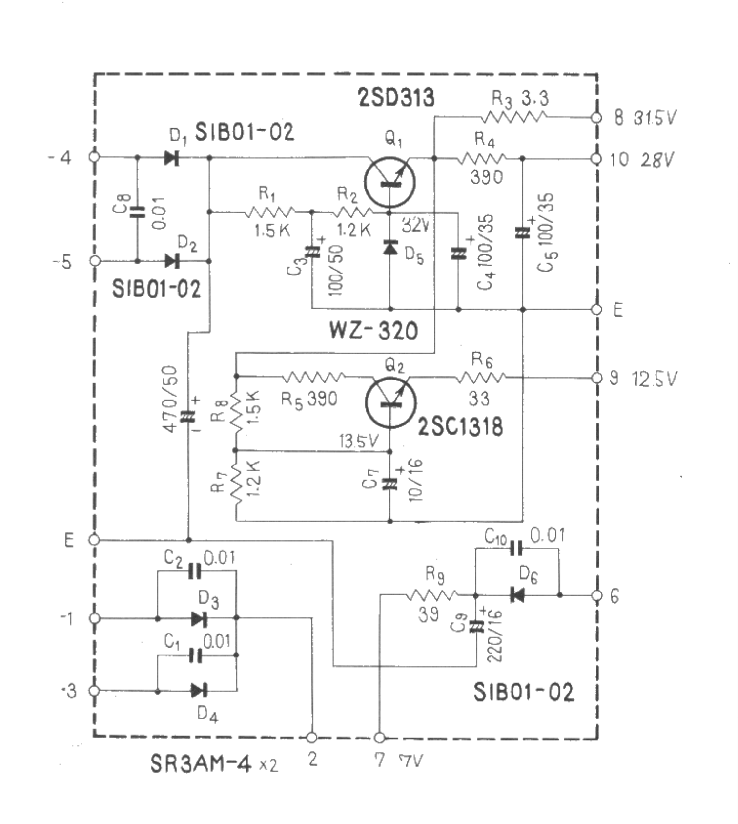
Power supply ass'y AWR-021
