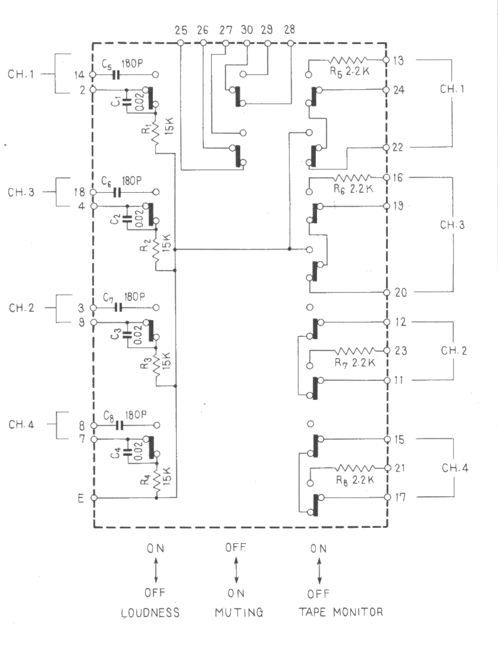
Switch ass'y AWS-023
