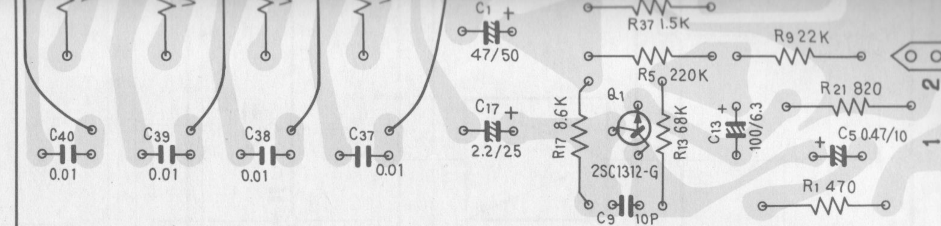
Decoder ass'y AWM-031
