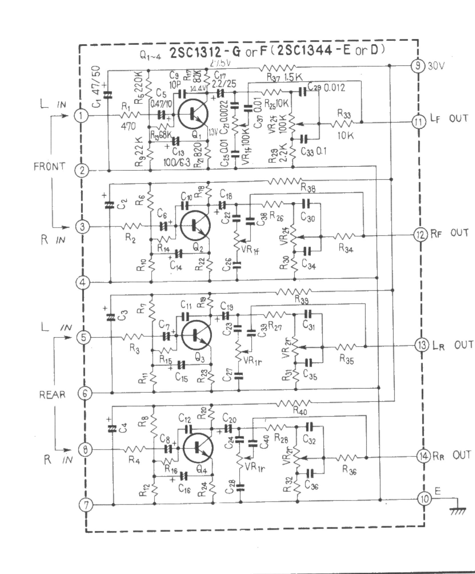
Control amp ass'y AWG-015
