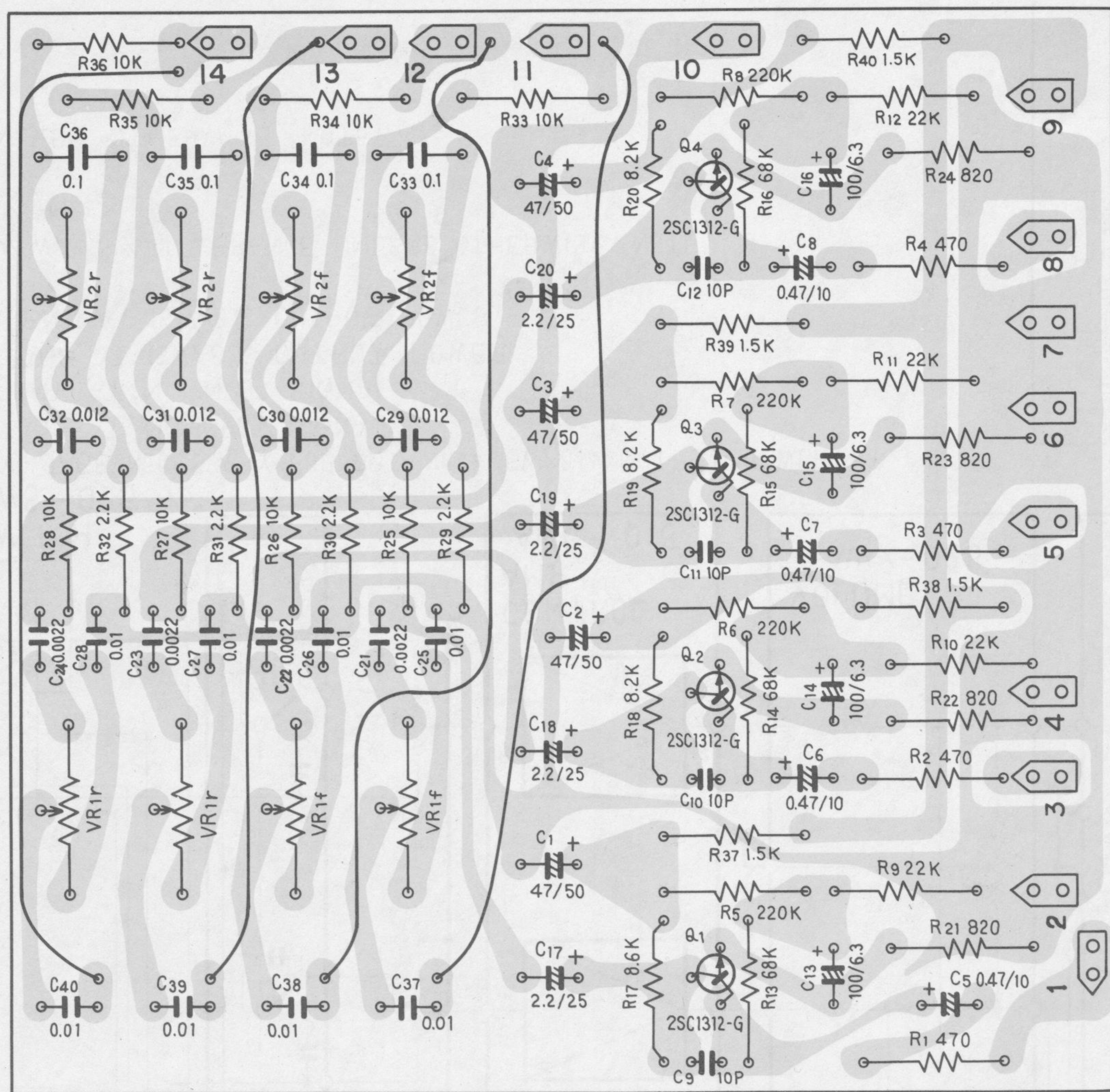
Control amp ass'y AWP-015
