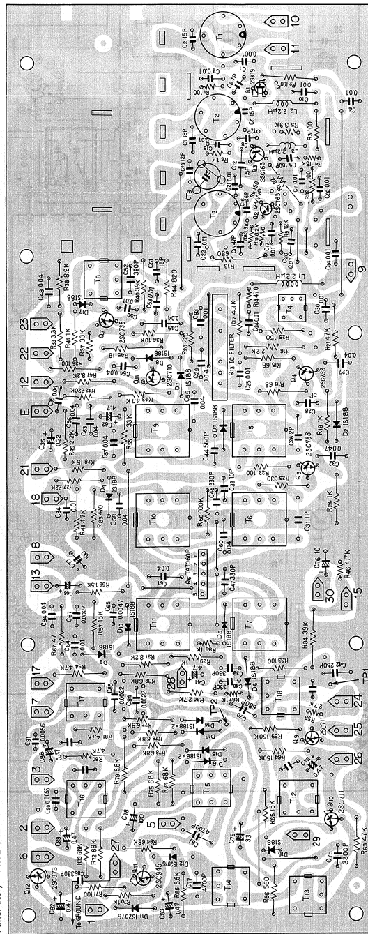
Tuner ass'y AWE-012
