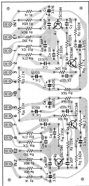
Head amp ass'y AWF-003
