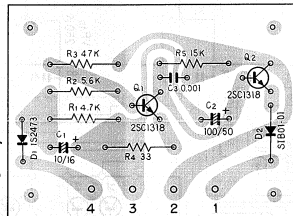
Muting ass'y AWM-033
