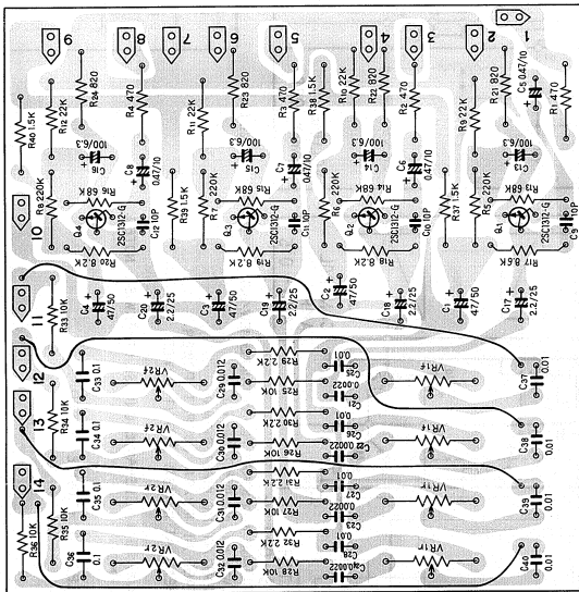
Control amp ass'y AWW-015
