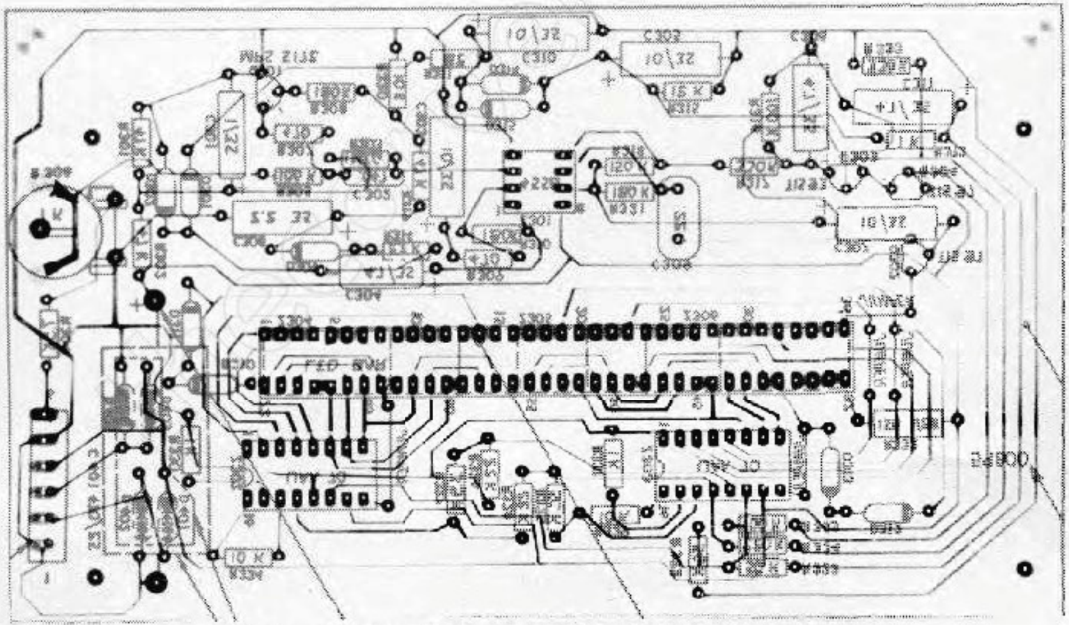
Diagram 2-6. X-ray view of PL37, from foil side.
