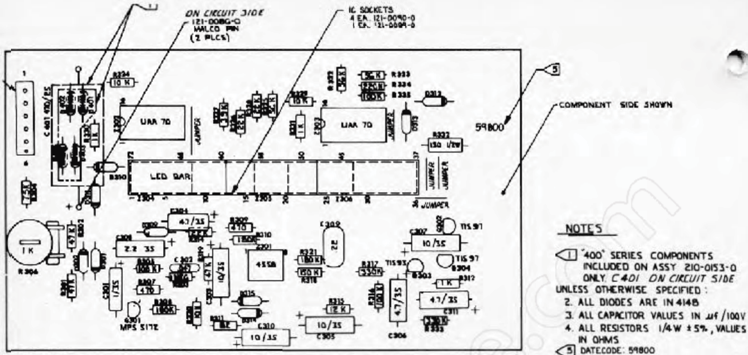
PL 37 PCB ASSY
