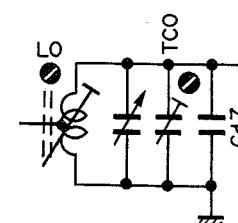
Fig. 4.1.10 Dial Calibration
