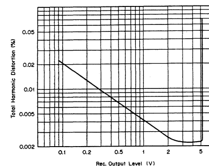
Output vs. Total Harmonic Distortion (Phono Amp.) Frequency: 1 kHz Output: Recording Output
