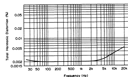
Aux. Input vs. Total Harmonic Distortion Rec. Output: 2 V Constant
