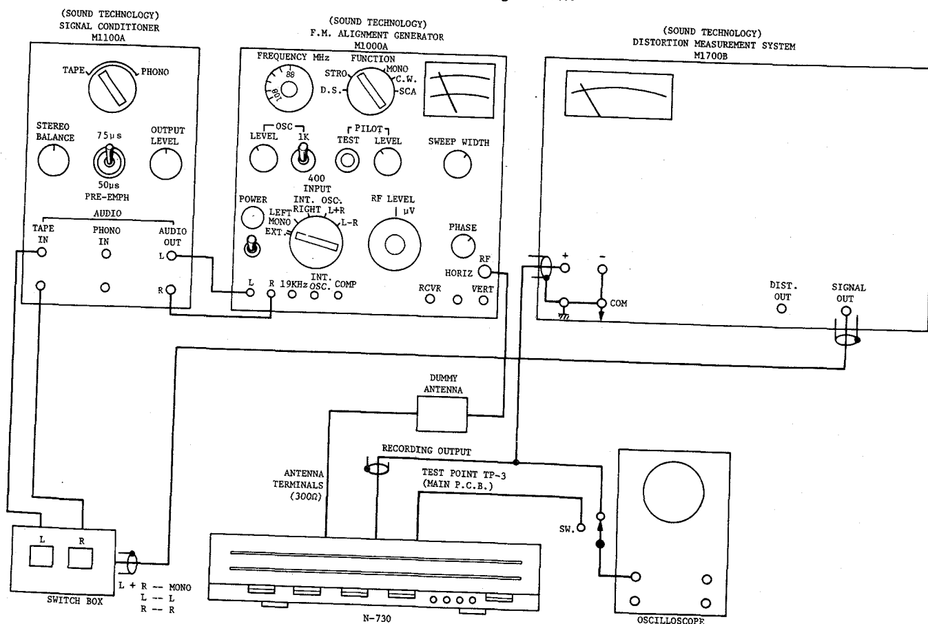
Fig. 4.1.1 Connection Diagram
