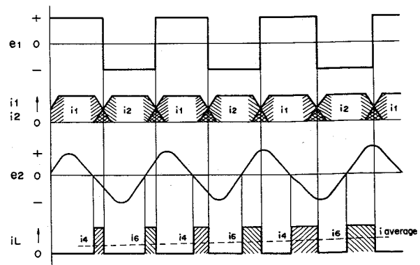
Fig. 2.1.27 Timing Chart
