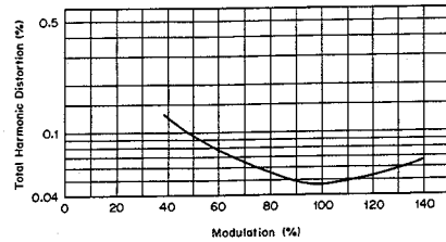
Modulation vs. Total Harmonic Distortion Modulation: Main 45.5 % Sub-carrier 45.5 % Pilot 9 % Frequency: 1 kHz Antenna Input: 98 MHz, 65 dBf, 1 mV, 300 \Omega
