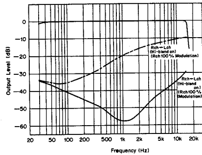
Stereo Separation Antenna Input: 98 MHz, 65 dBf, 1 mV, 300 \Omega
