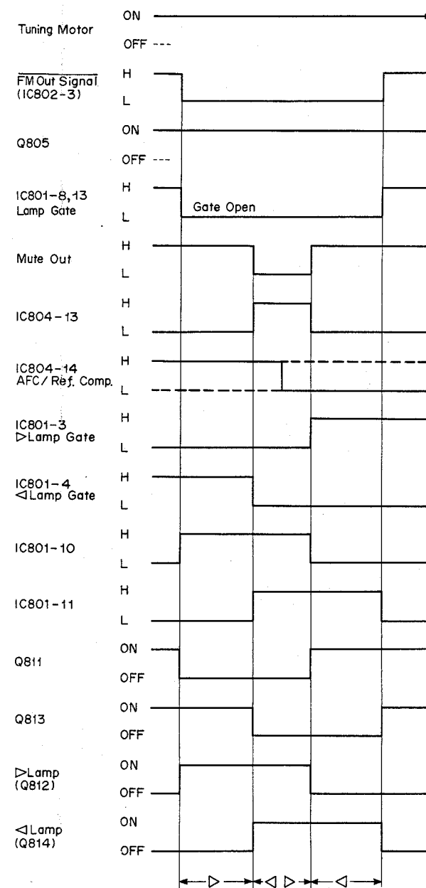
Fig. 2.4.14 Preset Tuning Timing Chart
