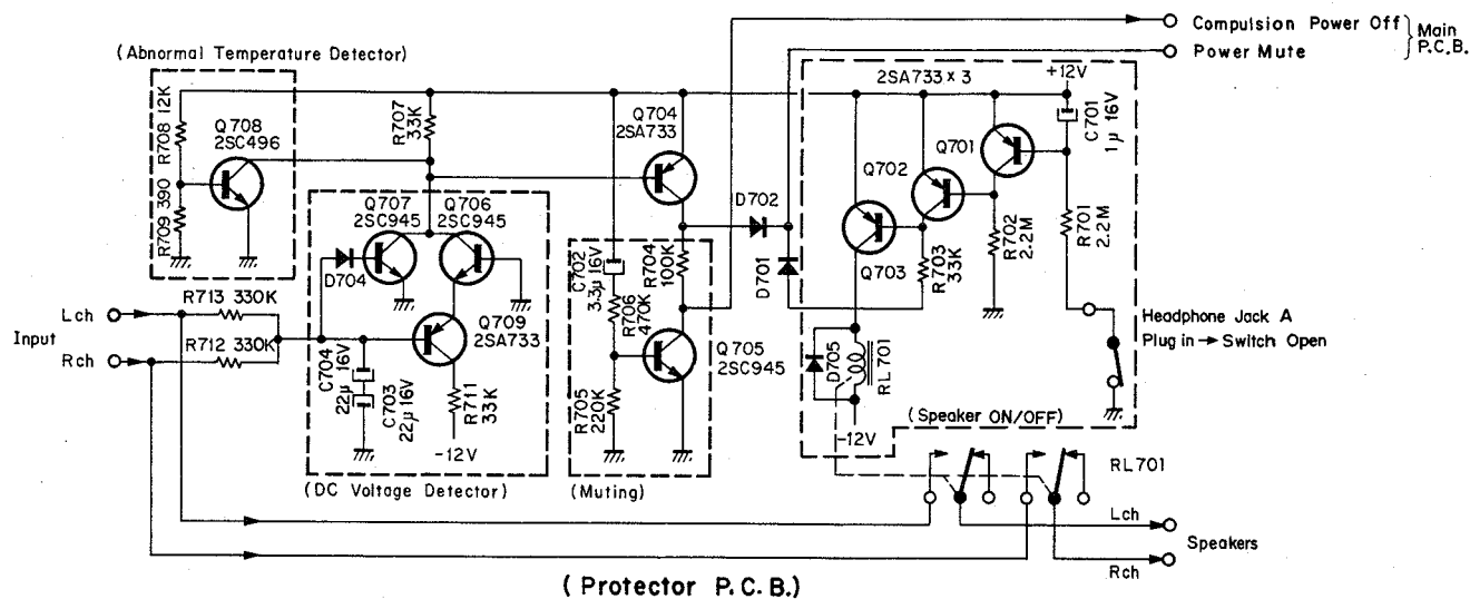
Fig. 2.5.14 Protector Circuit
