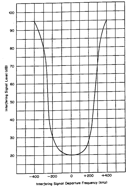
Channel Selectivity Impedance: 300 \Omega Interfering Signal: 1 kHz, 100 % Modulation Interference Output Level: -30 dB Desired Signal: Unmodulated
