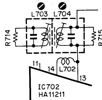
Fig. 4.1.5 DC Balance, Distortion (Mono)
