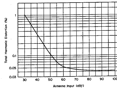
Input vs. Total Harmonic Distortion (Stereo) Antenna Input: 98 MHz, 1 mV, 300 \Omega Modulation: Main 45.5 % Sub-carrier 45.5 % Pilot 9 %
