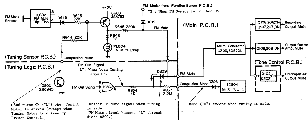
Fig. 2.4.16 FM Mute and Compulsion Mono
