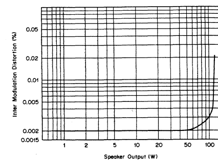
Output vs. I.M. Distortion (Power Amp.) Load Impedance: 8 \Omega Input Signal: 60 Hz : 7 kHz = 4 : 1
