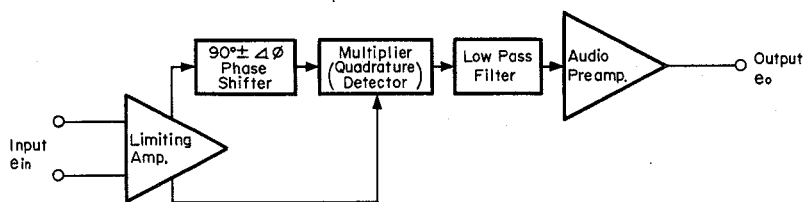
Fig. 2.1.25 Quadrature Detector System Diagram
