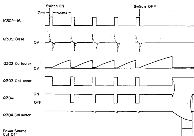
Fig. 2.6.5 Timing Chart
