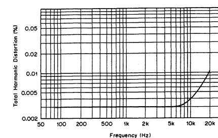
Input vs. Total Harmonic Distortion (Phono Amp.) Rec. Output: 2 V Constant
