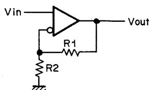
Fig. 2.1.14 Non-inverting
