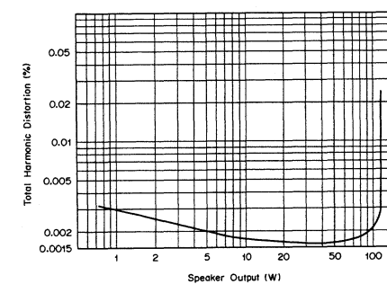
Output vs. Total Harmonic Distortion (Power Amp.) Frequency: 1 kHz Load Impedance: 8 \Omega
