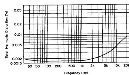
Frequency vs. Total Harmonic Distortion (Power Amp.) Load Impedance: 8 \Omega Output: 50 W Constant
