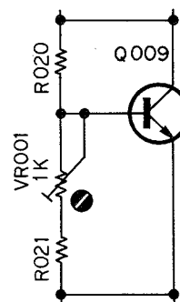
Fig. 4.3.2 Idling Current Adjustment
