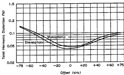
Tuning vs. Total Harmonic Distortion Antenna Input: 98 MHz, 65 dBf, 1 mV, 300 \Omega Modulation: Main 45.5 % Sub-carrier 45.5 % Pilot 9 %
