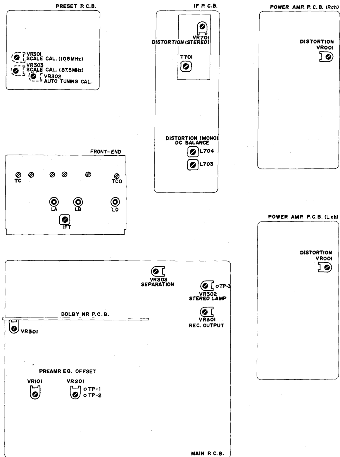
Fig. 4.1.2 Diagram for Adjustment
