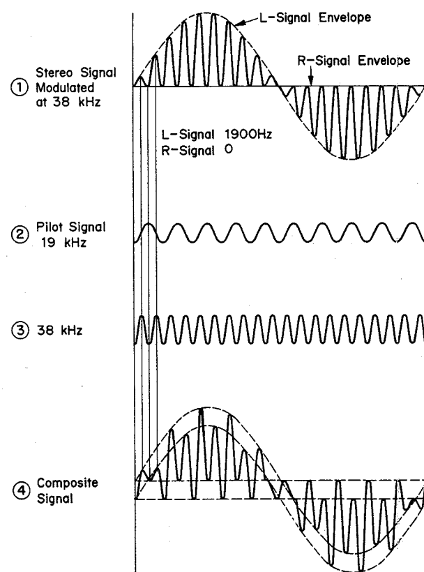
Fig. 2.4.2 MPX Stereo Signal
