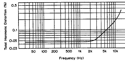
Frequency vs. Total Harmonic Distortion Antenna Input: 98 MHz, 65 dBf, 1 mV, 300 \Omega Modulation: Main 45.5 % Sub-carrier 45.5 % Pilot 9 %
