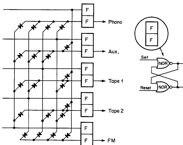
Fig. 2.1.10 5-Way Switch
