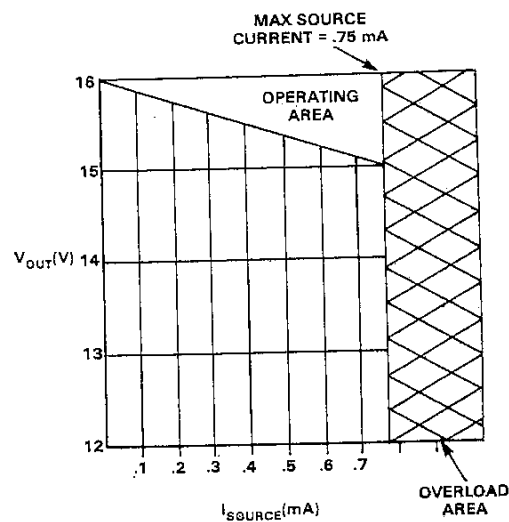
OUTPUT SOURCE CHARACTERISTICS
