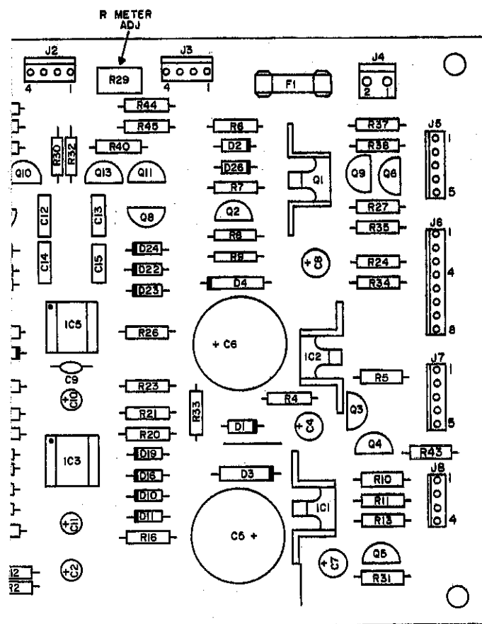
METER/REGULATOR PCB 047190
