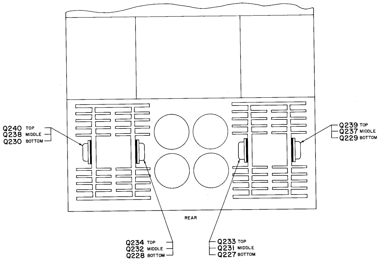
LOCATION OF TRANSISTORS NOT ON PC BOARD
