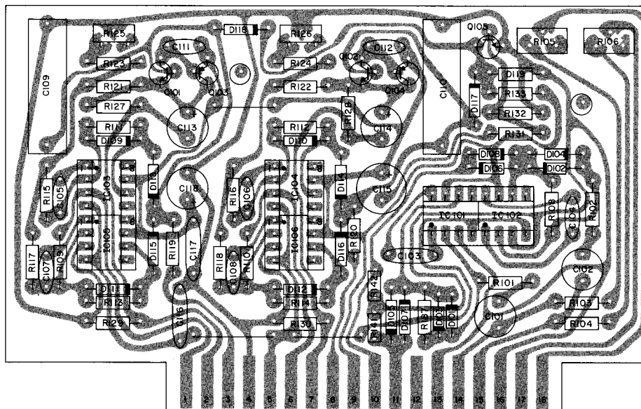
METER PC BOARD 044-624
